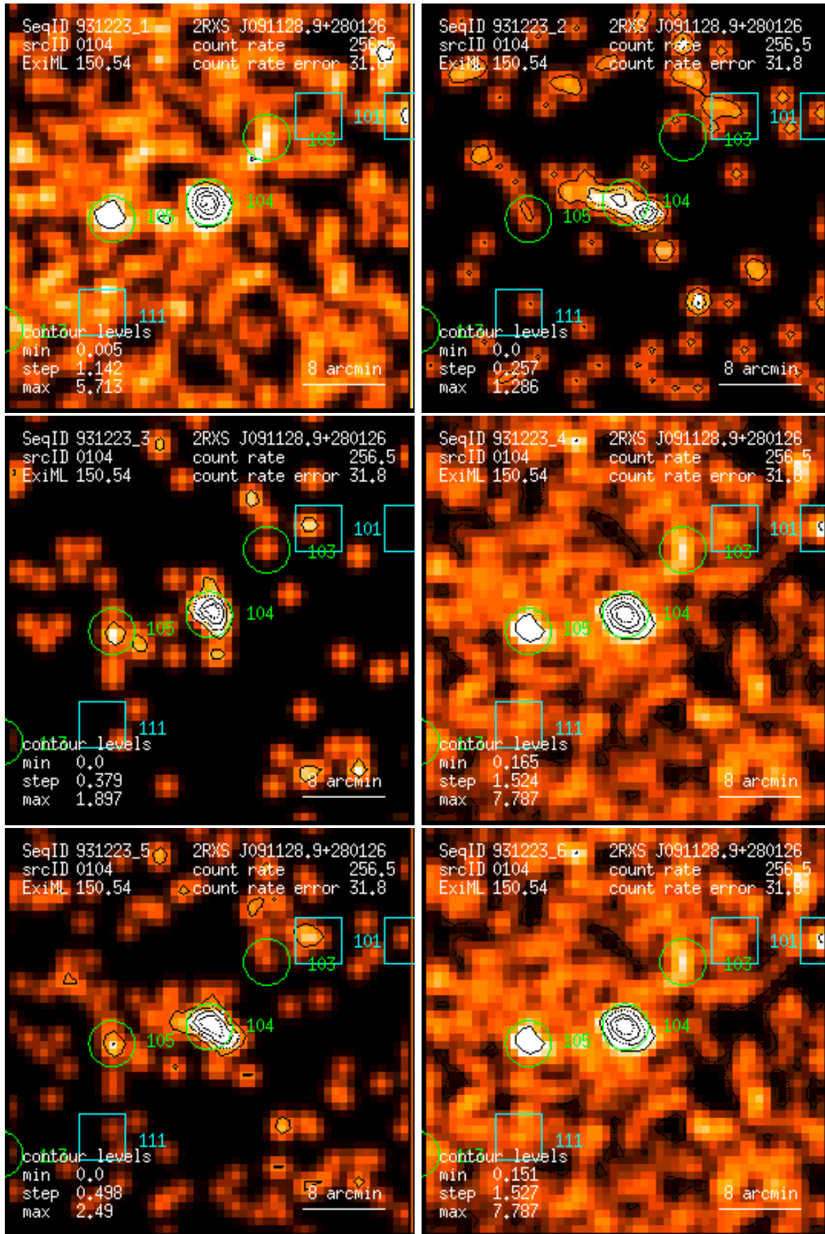
Figure 104: RASS 931223: detection 0104: band rate images, Gaussian filter: (1) PSPC channels 11 – 41, (2) 52 – 90, (3) 91 – 201, (4) 11 – 235, (5) 52 – 201, (6) 11 – 201. Broad band rates in counts/ks. Band rate contour levels in counts/ks/arcmin 2 .
