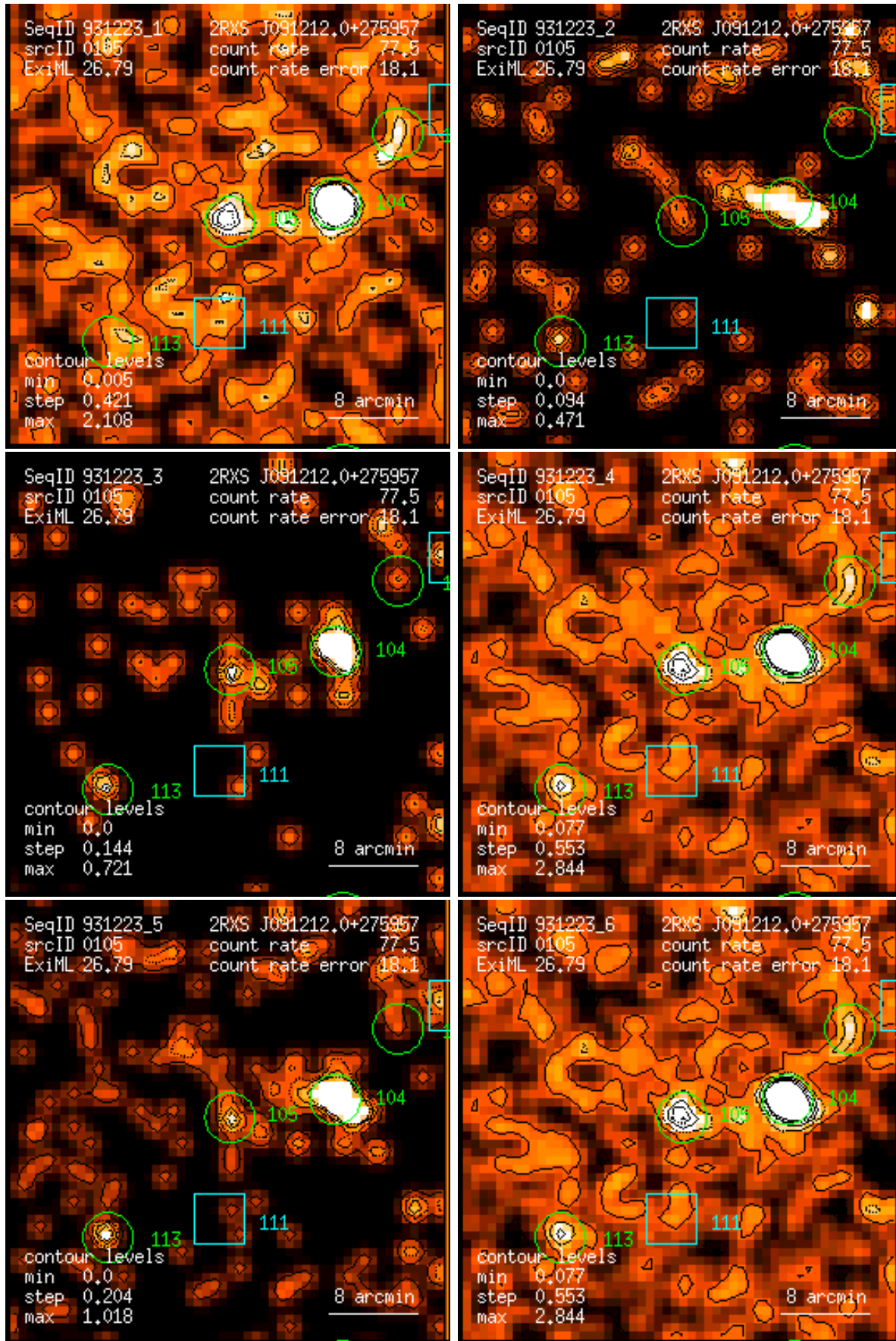
Figure 105: RASS 931223: detection 0105: band rate images, Gaussian filter: (1) PSPC channels 11 – 41, (2) 52 – 90, (3) 91 – 201, (4) 11 – 235, (5) 52 – 201, (6) 11 – 201. Broad band rates in counts/ks. Band rate contour levels in counts/ks/arcmin 2 .
