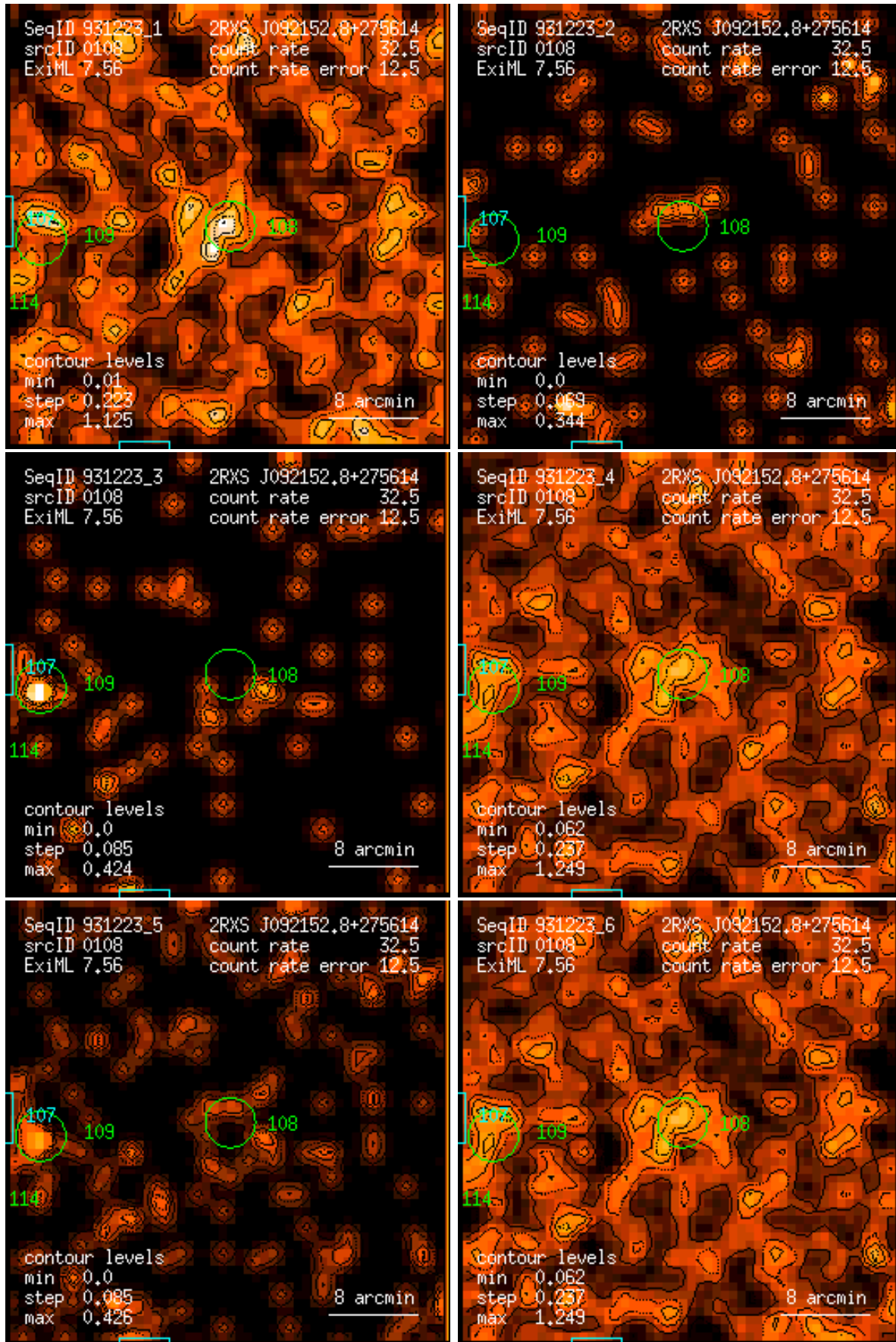
Figure 108: RASS 931223: detection 0108: band rate images, Gaussian filter: (1) PSPC channels 11 – 41, (2) 52 – 90, (3) 91 – 201, (4) 11 – 235, (5) 52 – 201, (6) 11 – 201. Broad band rates in counts/ks. Band rate contour levels in counts/ks/arcmin 2 .
