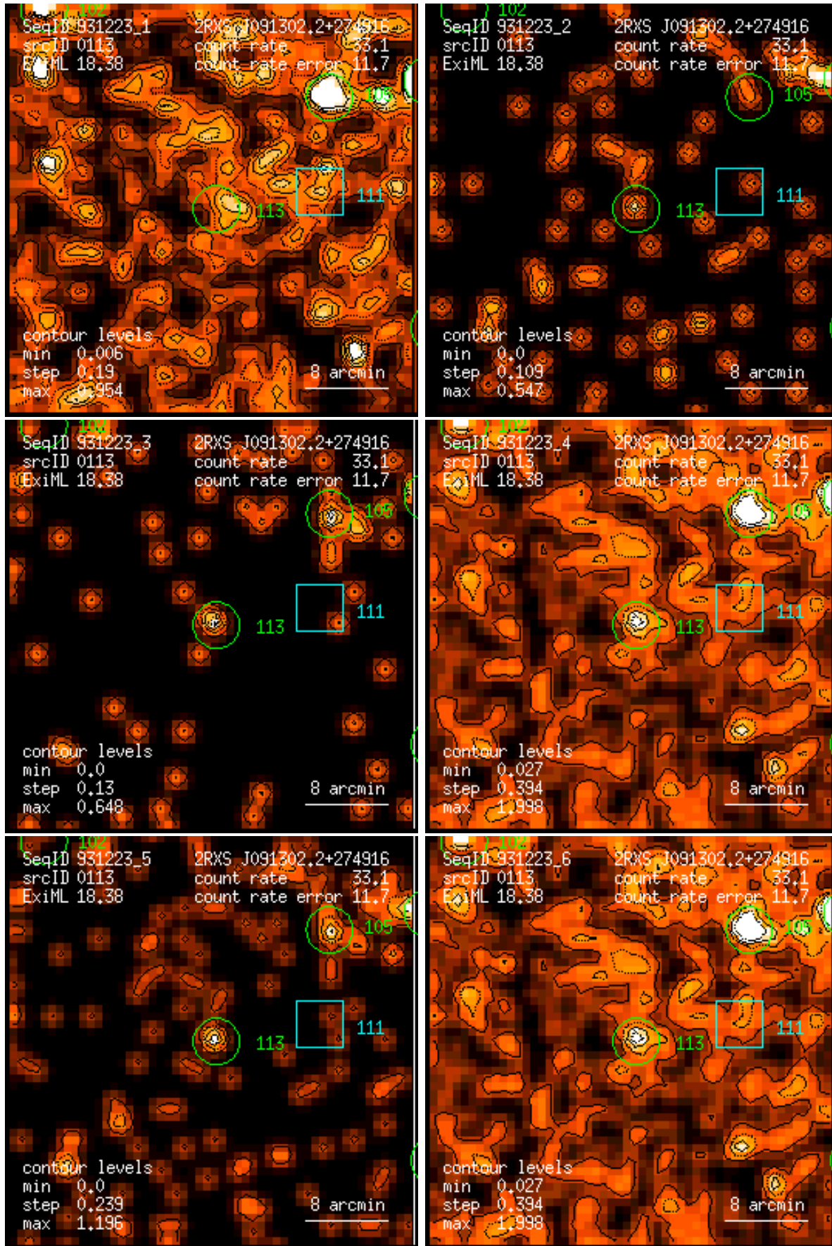
Figure 113: RASS 931223: detection 0113: band rate images, Gaussian filter: (1) PSPC channels 11 – 41, (2) 52 – 90, (3) 91 – 201, (4) 11 – 235, (5) 52 – 201, (6) 11 – 201. Broad band rates in counts/ks. Band rate contour levels in counts/ks/arcmin 2 .
