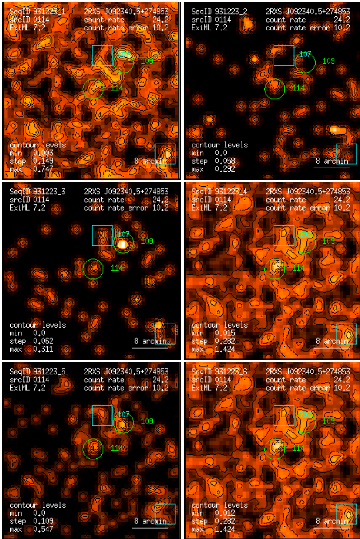
Figure 114: RASS 931223: detection 0114: band rate images, Gaussian filter: (1) PSPC channels 11 – 41, (2) 52 – 90, (3) 91 – 201, (4) 11 – 235, (5) 52 – 201, (6) 11 – 201. Broad band rates in counts/ks. Band rate contour levels in counts/ks/arcmin 2 .
