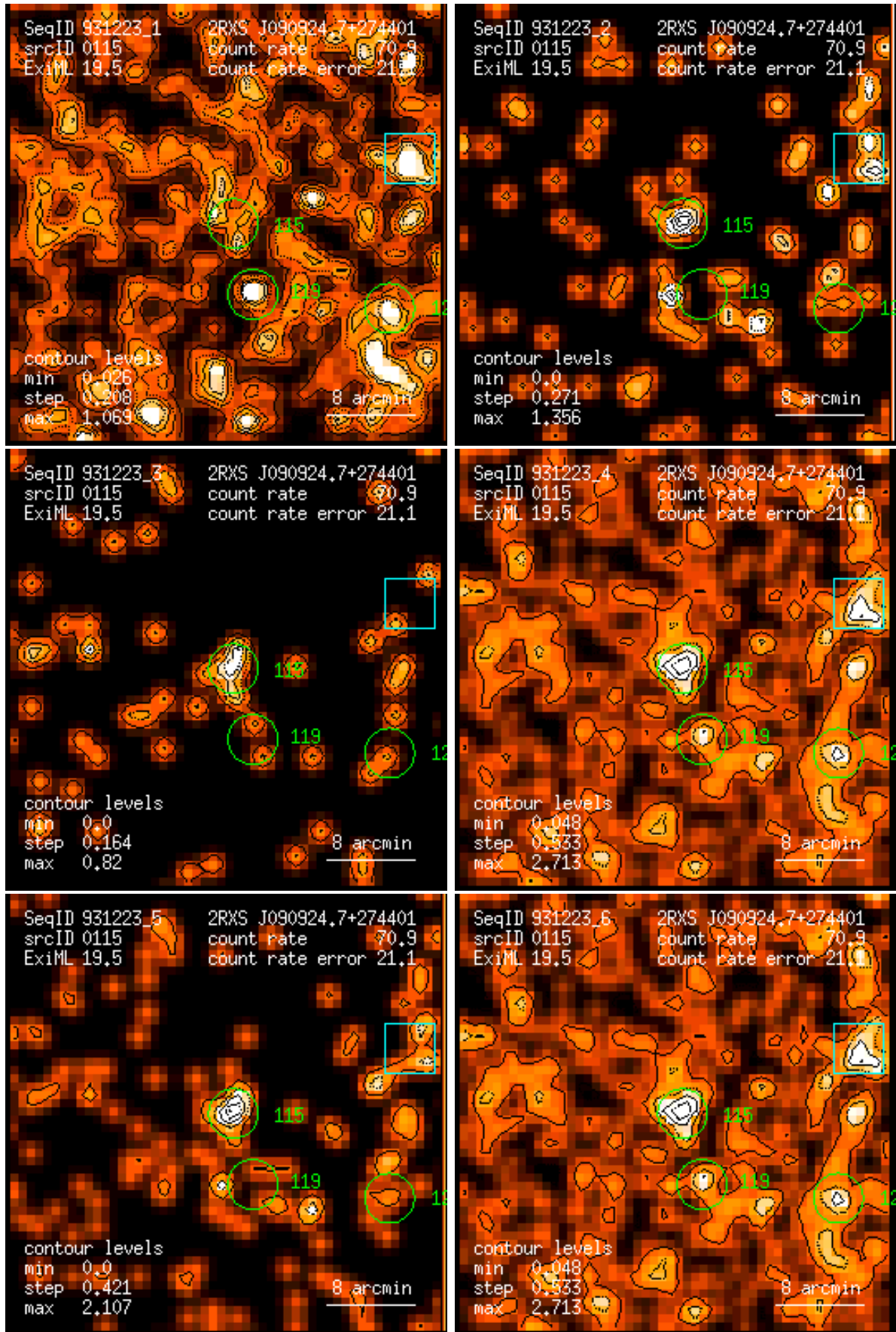
Figure 115: RASS 931223: detection 0115: band rate images, Gaussian filter: (1) PSPC channels 11 – 41, (2) 52 – 90, (3) 91 – 201, (4) 11 – 235, (5) 52 – 201, (6) 11 – 201. Broad band rates in counts/ks. Band rate contour levels in counts/ks/arcmin 2 .
