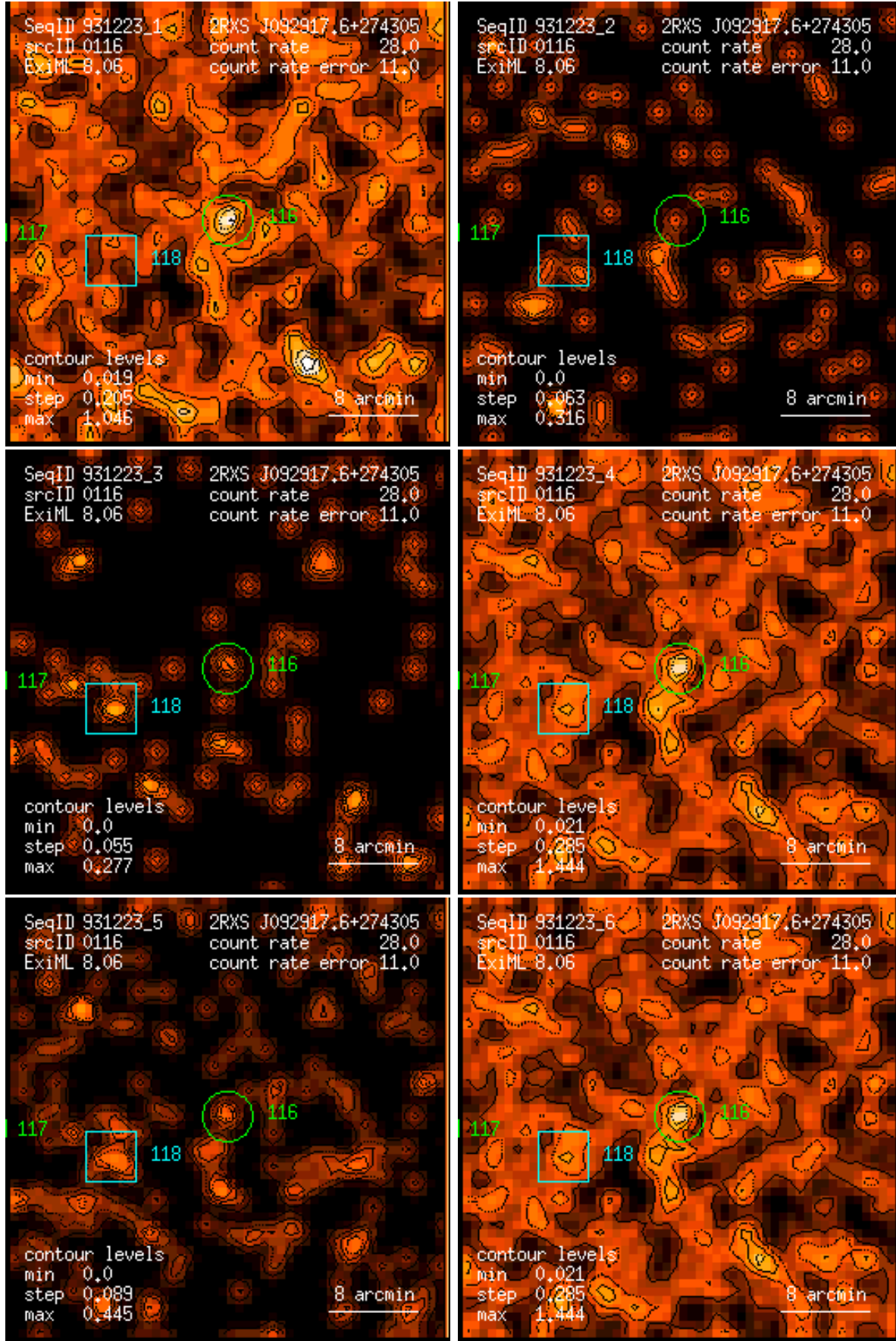
Figure 116: RASS 931223: detection 0116: band rate images, Gaussian filter: (1) PSPC channels 11 – 41, (2) 52 – 90, (3) 91 – 201, (4) 11 – 235, (5) 52 – 201, (6) 11 – 201. Broad band rates in counts/ks. Band rate contour levels in counts/ks/arcmin 2 .
