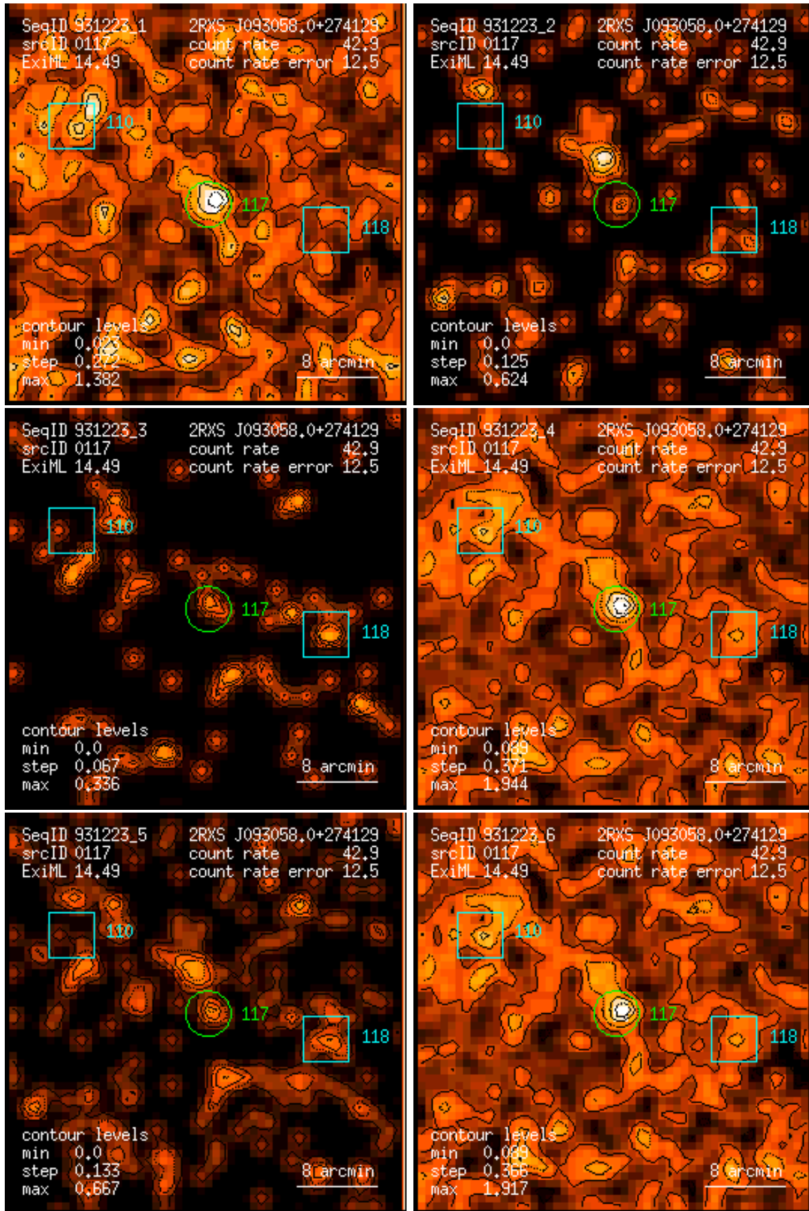
Figure 117: RASS 931223: detection 0117: band rate images, Gaussian filter: (1) PSPC channels 11 – 41, (2) 52 – 90, (3) 91 – 201, (4) 11 – 235, (5) 52 – 201, (6) 11 – 201. Broad band rates in counts/ks. Band rate contour levels in counts/ks/arcmin 2 .
