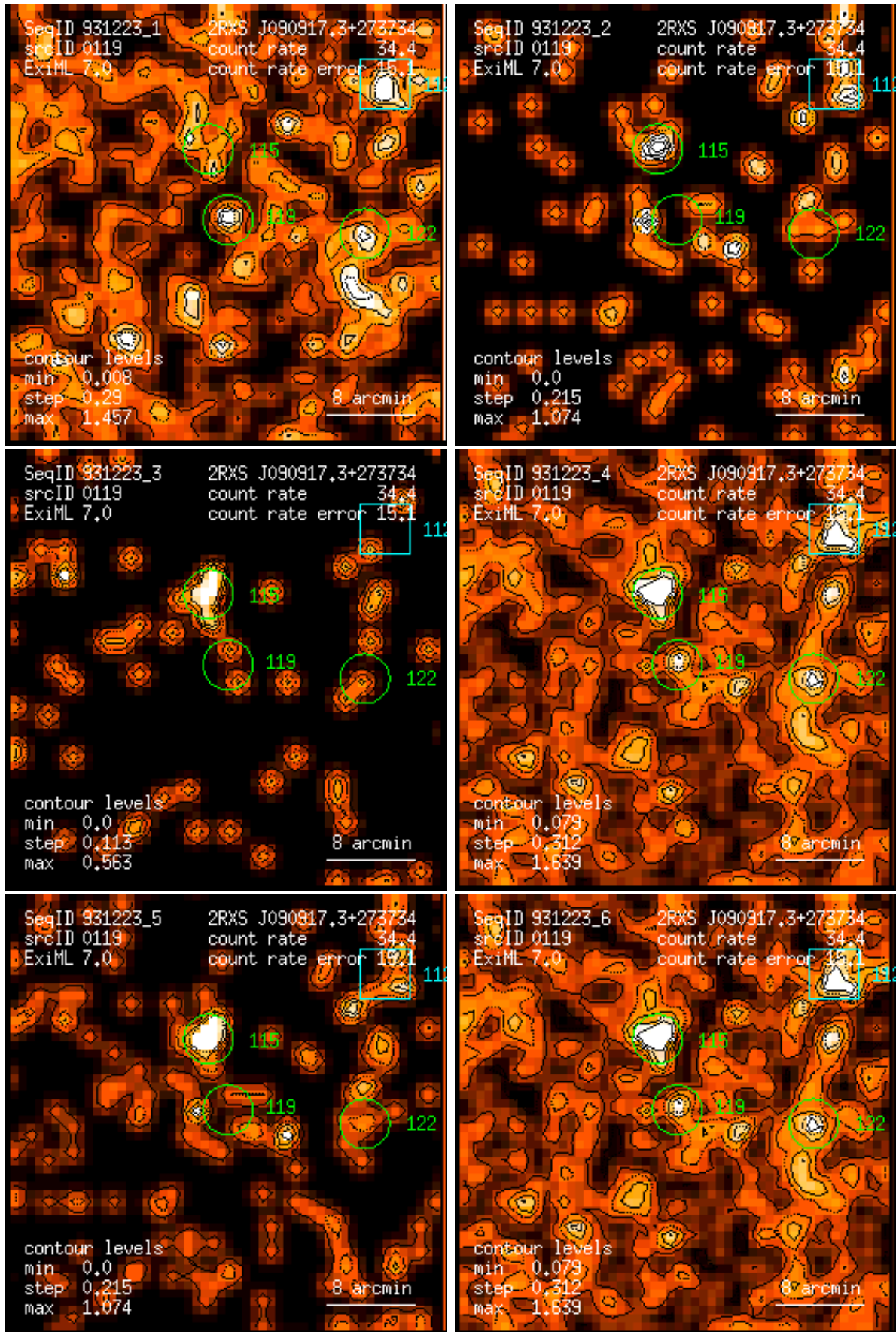
Figure 119: RASS 931223: detection 0119: band rate images, Gaussian filter: (1) PSPC channels 11 – 41, (2) 52 – 90, (3) 91 – 201, (4) 11 – 235, (5) 52 – 201, (6) 11 – 201. Broad band rates in counts/ks. Band rate contour levels in counts/ks/arcmin 2 .
