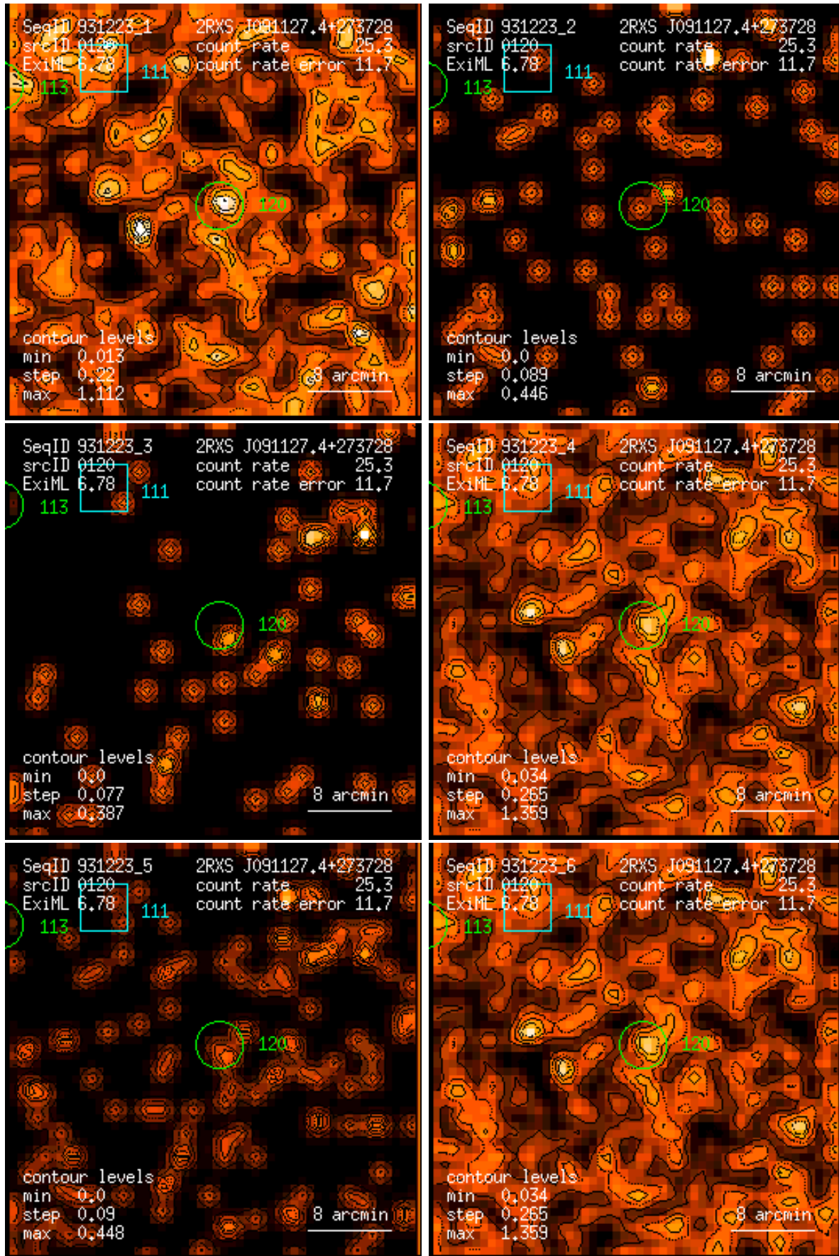
Figure 120: RASS 931223: detection 0120: band rate images, Gaussian filter: (1) PSPC channels 11 – 41, (2) 52 – 90, (3) 91 – 201, (4) 11 – 235, (5) 52 – 201, (6) 11 – 201. Broad band rates in counts/ks. Band rate contour levels in counts/ks/arcmin 2 .
