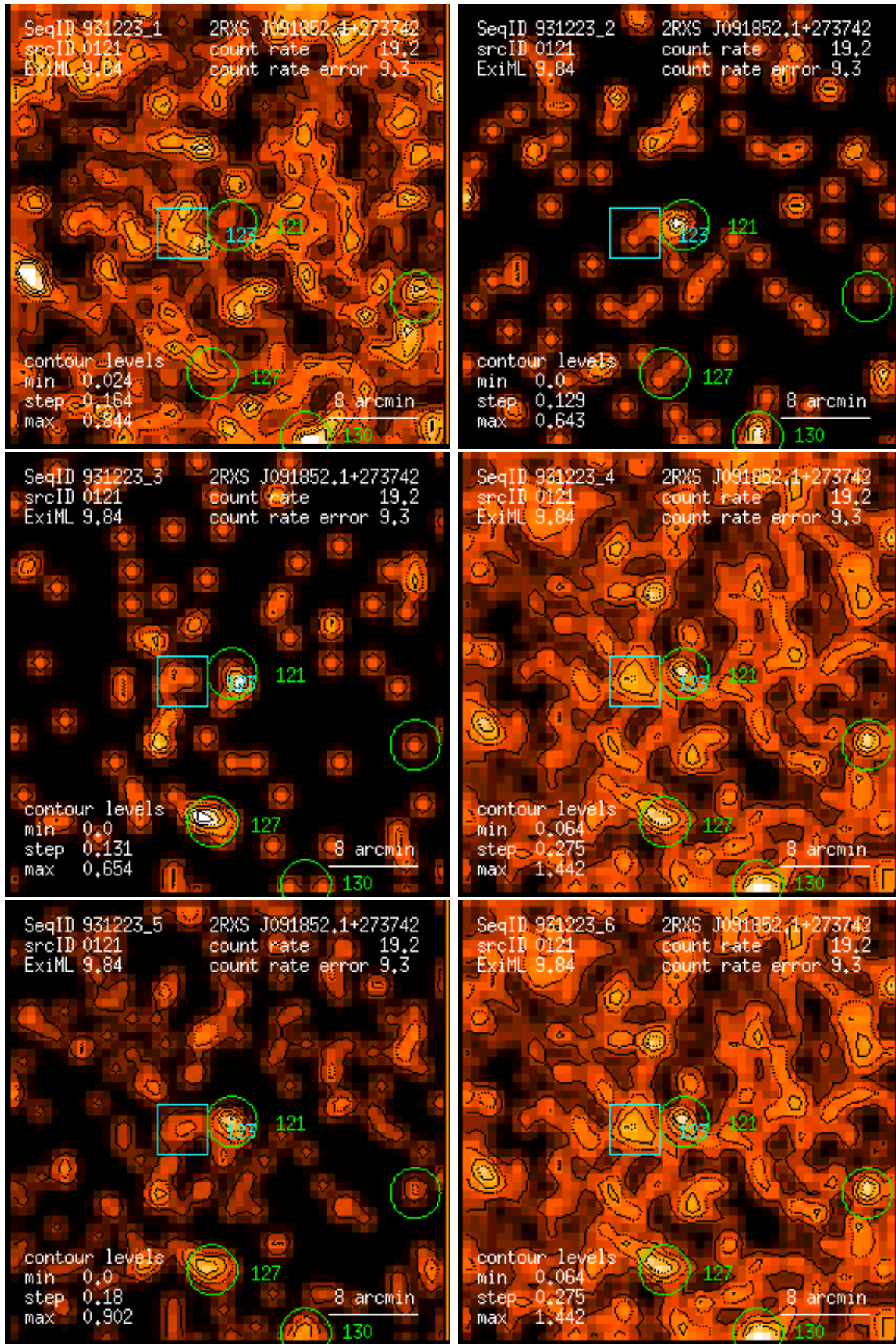
Figure 121: RASS 931223: detection 0121: band rate images, Gaussian filter: (1) PSPC channels 11 – 41, (2) 52 – 90, (3) 91 – 201, (4) 11 – 235, (5) 52 – 201, (6) 11 – 201. Broad band rates in counts/ks. Band rate contour levels in counts/ks/arcmin 2 .
