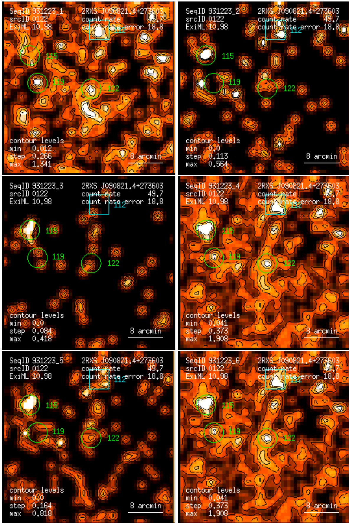
Figure 122: RASS 931223: detection 0122: band rate images, Gaussian filter: (1) PSPC channels 11 – 41, (2) 52 – 90, (3) 91 – 201, (4) 11 – 235, (5) 52 – 201, (6) 11 – 201. Broad band rates in counts/ks. Band rate contour levels in counts/ks/arcmin 2 .
