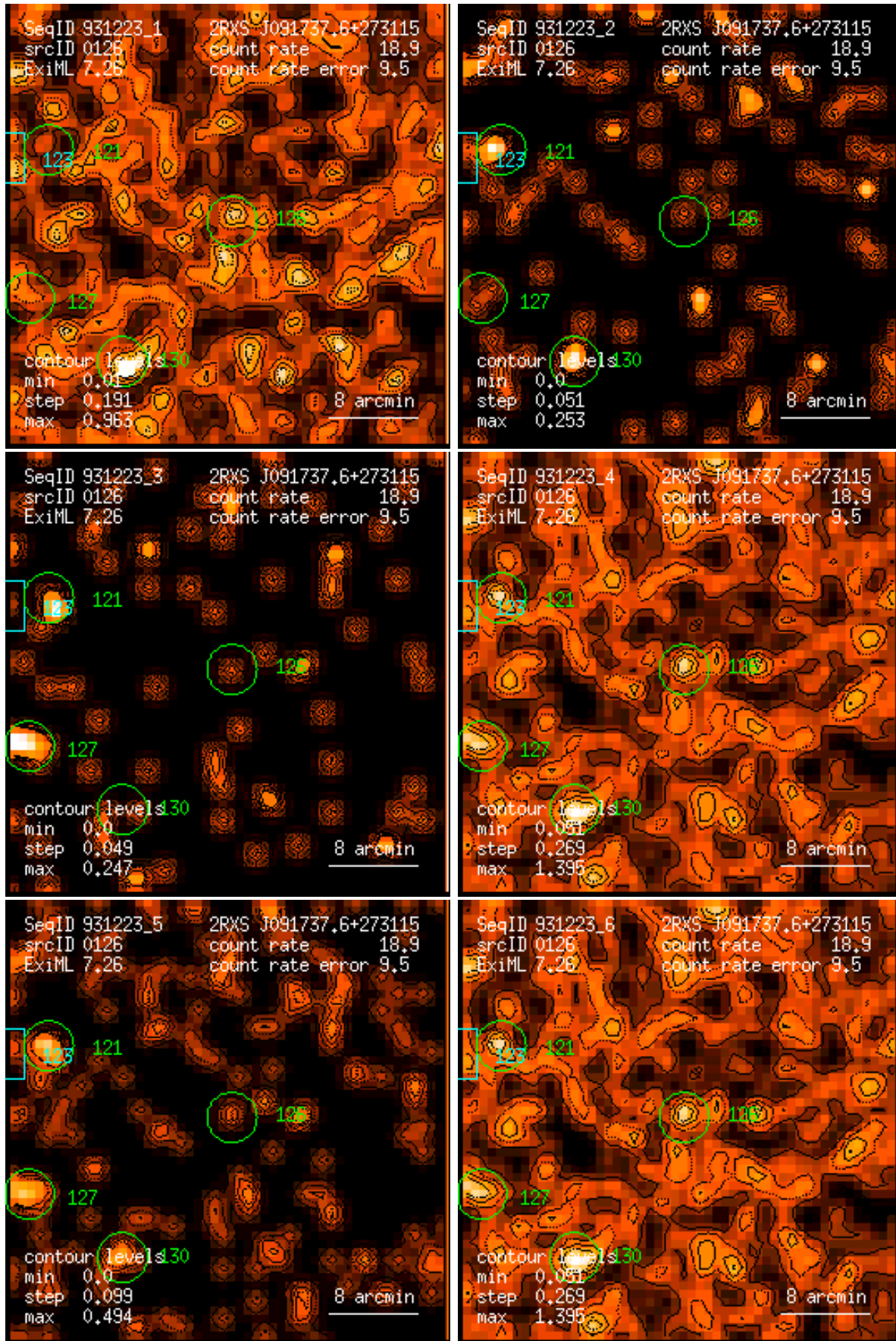
Figure 126: RASS 931223: detection 0126: band rate images, Gaussian filter: (1) PSPC channels 11 – 41, (2) 52 – 90, (3) 91 – 201, (4) 11 – 235, (5) 52 – 201, (6) 11 – 201. Broad band rates in counts/ks. Band rate contour levels in counts/ks/arcmin 2 .
