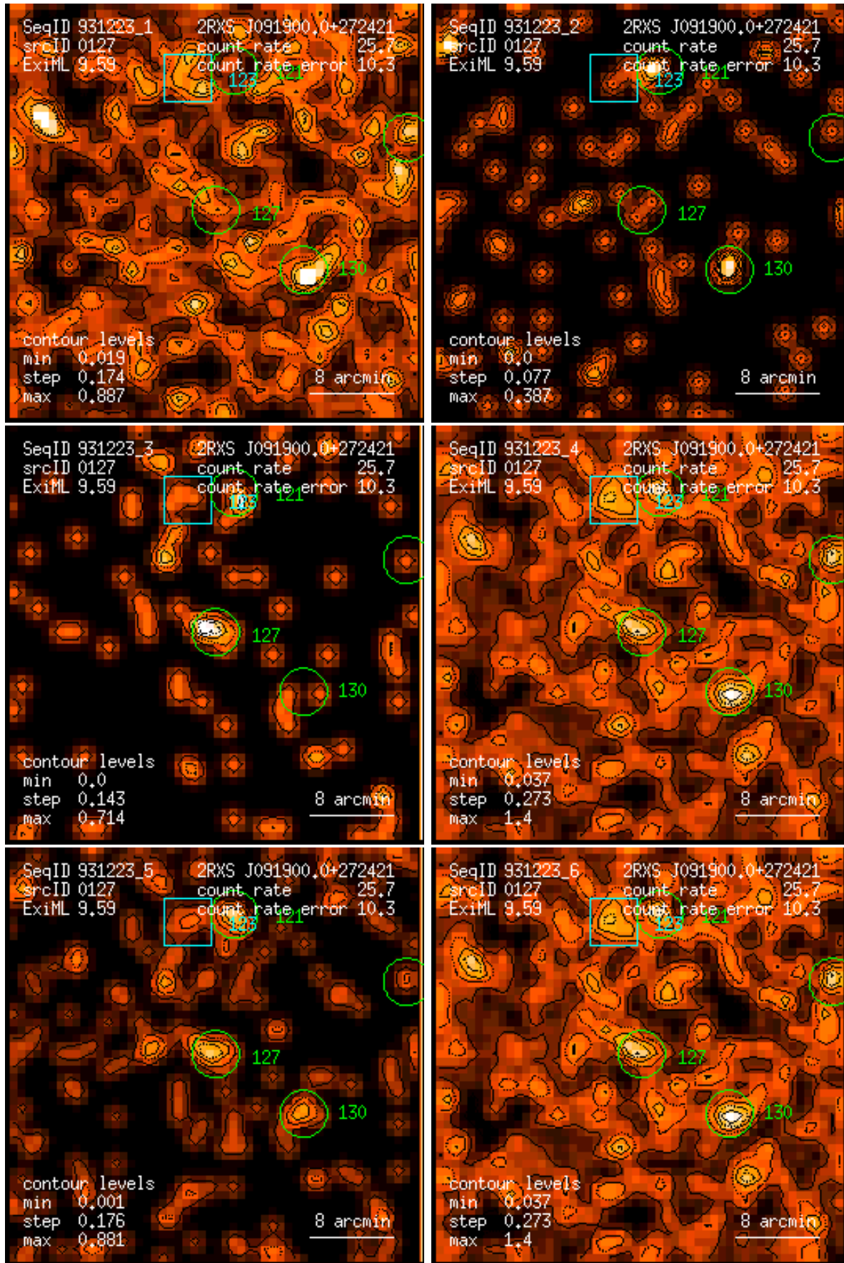
Figure 127: RASS 931223: detection 0127: band rate images, Gaussian filter: (1) PSPPC channels 11 – 41, (2) 52 – 90, (3) 91 – 201, (4) 11 – 235, (5) 52 – 201, (6) 11 – 201. Broad band rates in counts/ks. Band rate contour levels in counts/ks/arcmin 2 .
