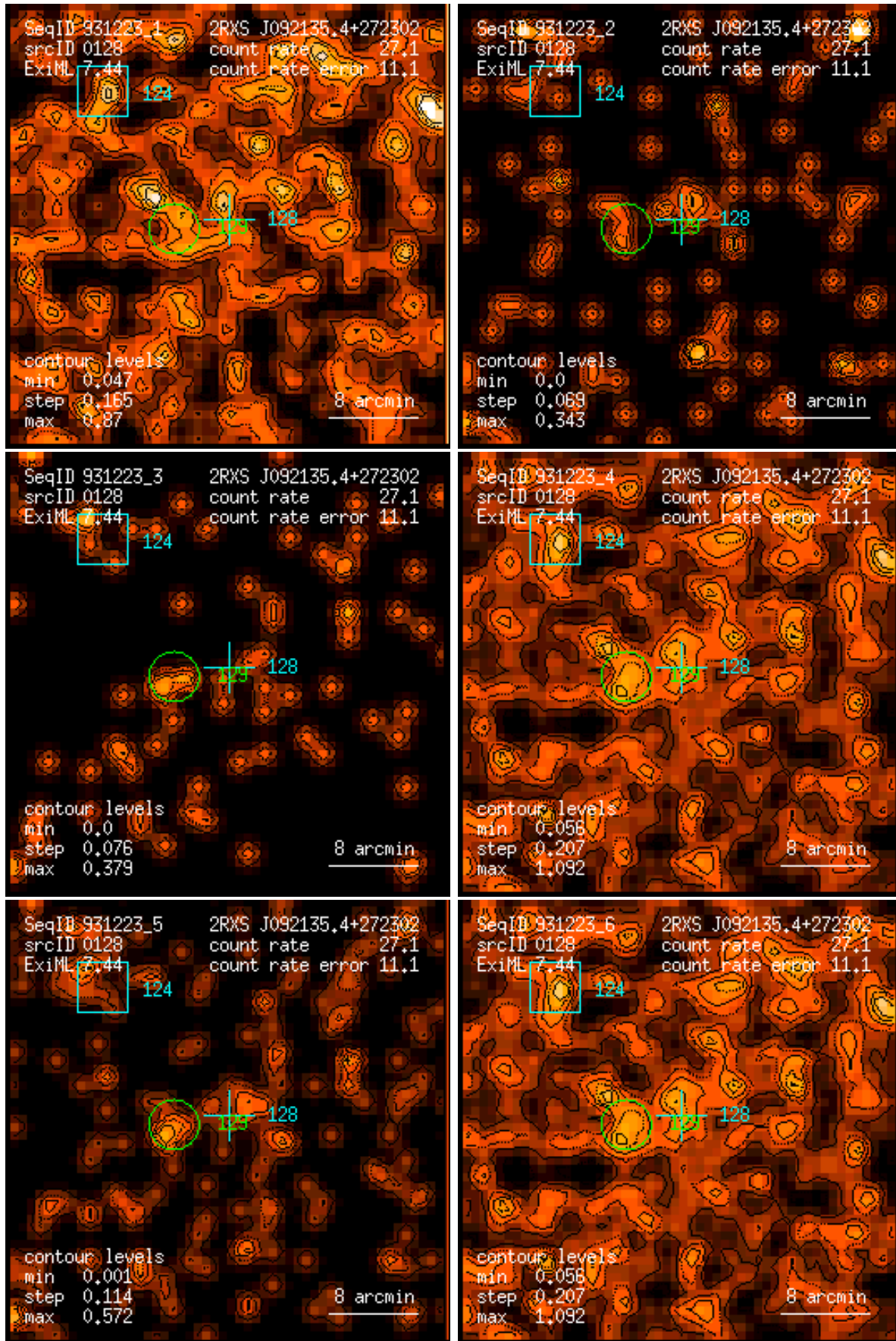
Figure 128: RASS 931223: detection 0128: band rate images, Gaussian filter: (1) PSPC channels 11 – 41, (2) 52 – 90, (3) 91 – 201, (4) 11 – 235, (5) 52 – 201, (6) 11 – 201. Broad band rates in counts/ks. Band rate contour levels in counts/ks/arcmin 2 .
