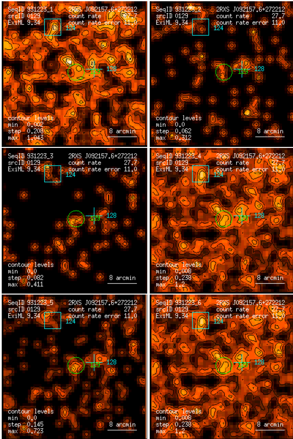
Figure 129: RASS 931223: detection 0129: band rate images, Gaussian filter: (1) PSPC channels 11 – 41, (2) 52 – 90, (3) 91 – 201, (4) 11 – 235, (5) 52 – 201, (6) 11 – 201. Broad band rates in counts/ks. Band rate contour levels in counts/ks/arcmin 2 .
