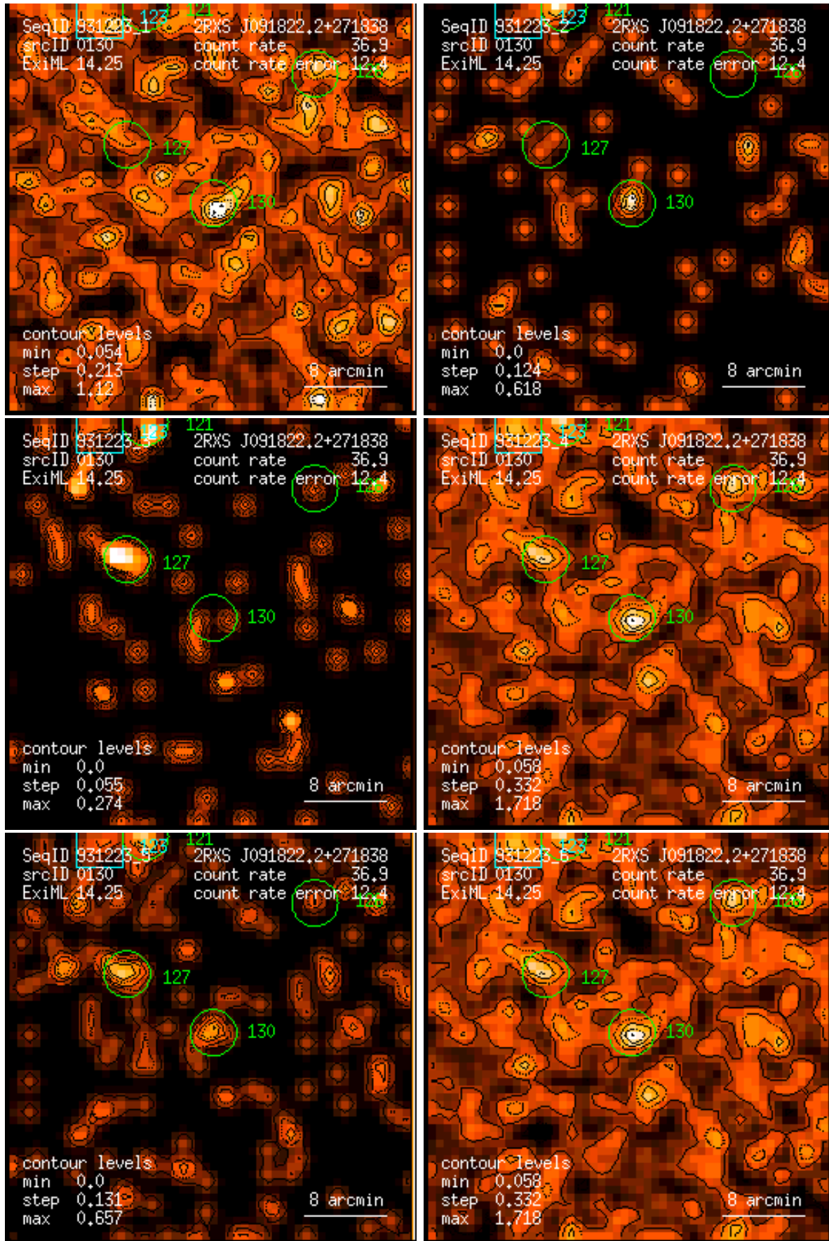
Figure 130: RASS 931223: detection 0130: band rate images, Gaussian filter: (1) PSPC channels 11 – 41, (2) 52 – 90, (3) 91 – 201, (4) 11 – 235, (5) 52 – 201, (6) 11 – 201. Broad band rates in counts/ks. Band rate contour levels in counts/ks/arcmin 2 .
