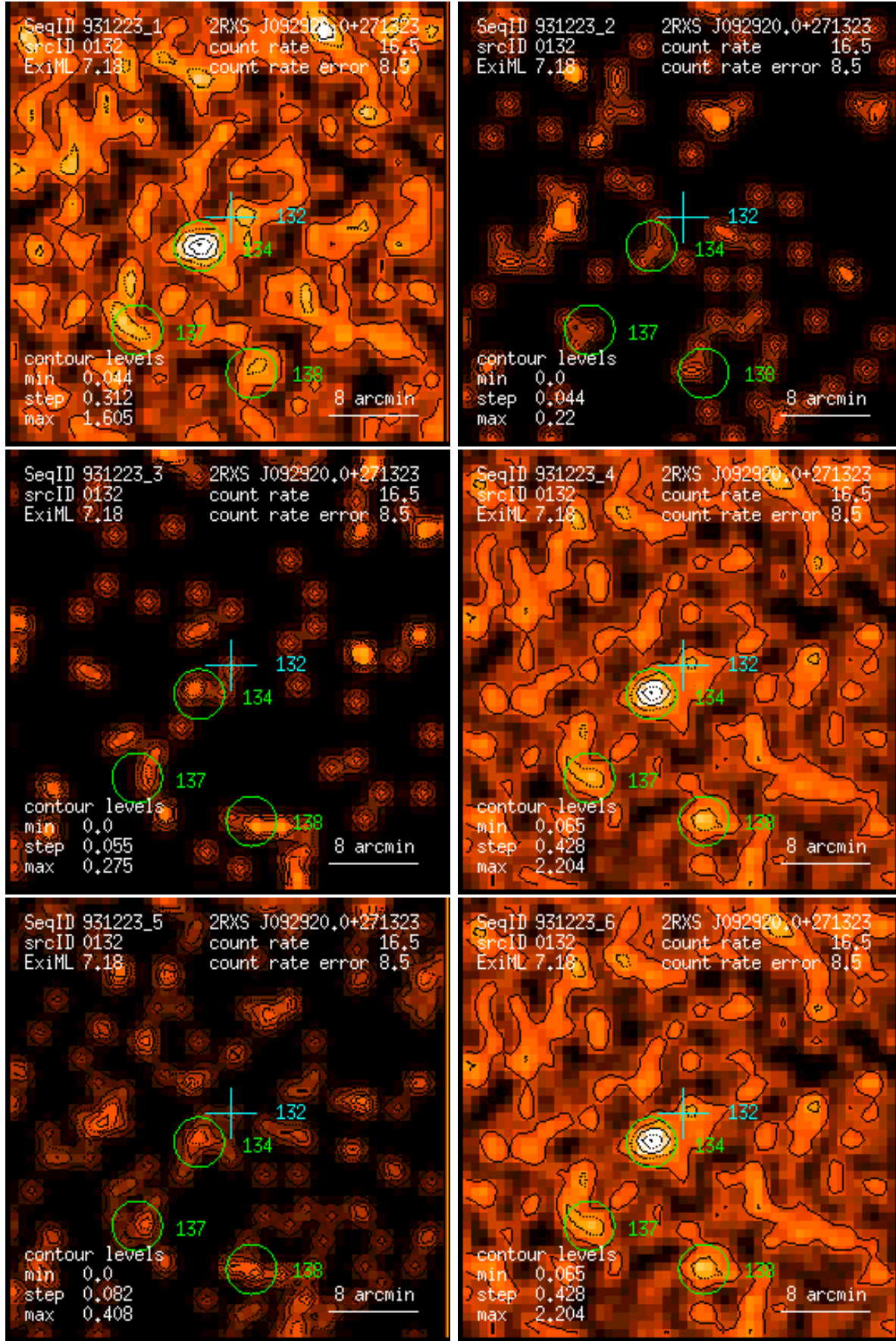
Figure 132: RASS 931223: detection 0132: band rate images, Gaussian filter: (1) PSPC channels 11 – 41, (2) 52 – 90, (3) 91 – 201, (4) 11 – 235, (5) 52 – 201, (6) 11 – 201. Broad band rates in counts/ks. Band rate contour levels in counts/ks/arcmin 2 .
