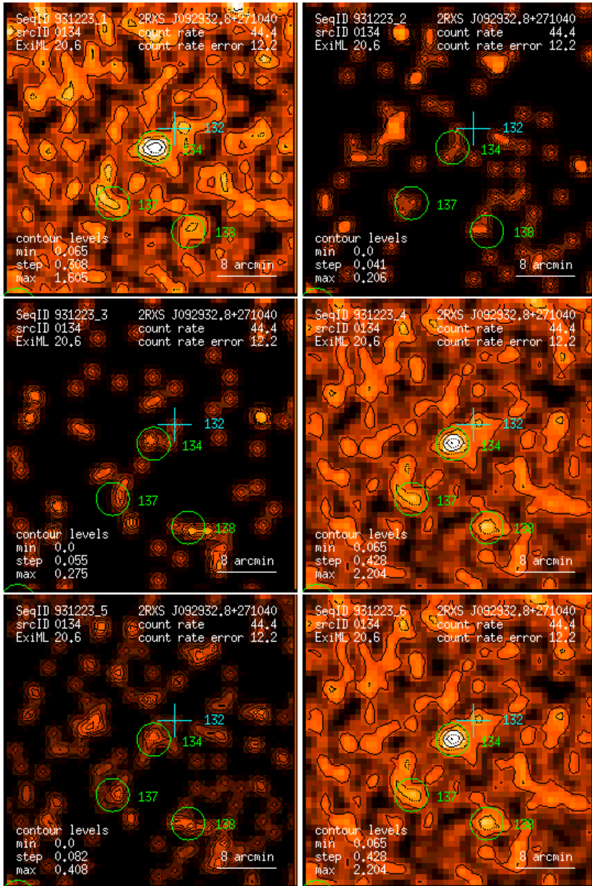
Figure 134: RASS 931223: detection 0134: band rate images, Gaussian filter: (1) PSPC channels 11 – 41, (2) 52 – 90, (3) 91 – 201, (4) 11 – 235, (5) 52 – 201, (6) 11 – 201. Broad band rates in counts/ks. Band rate contour levels in counts/ks/arcmin 2 .
