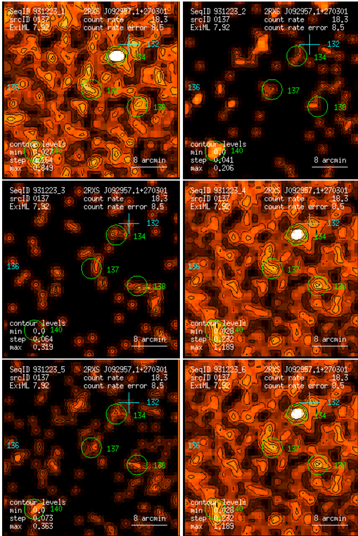
Figure 137: RASS 931223: detection 0137: band rate images, Gaussian filter: (1) PSPC channels 11 – 41, (2) 52 – 90, (3) 91 – 201, (4) 11 – 235, (5) 52 – 201, (6) 11 – 201. Broad band rates in counts/ks. Band rate contour levels in counts/ks/arcmin 2 .
