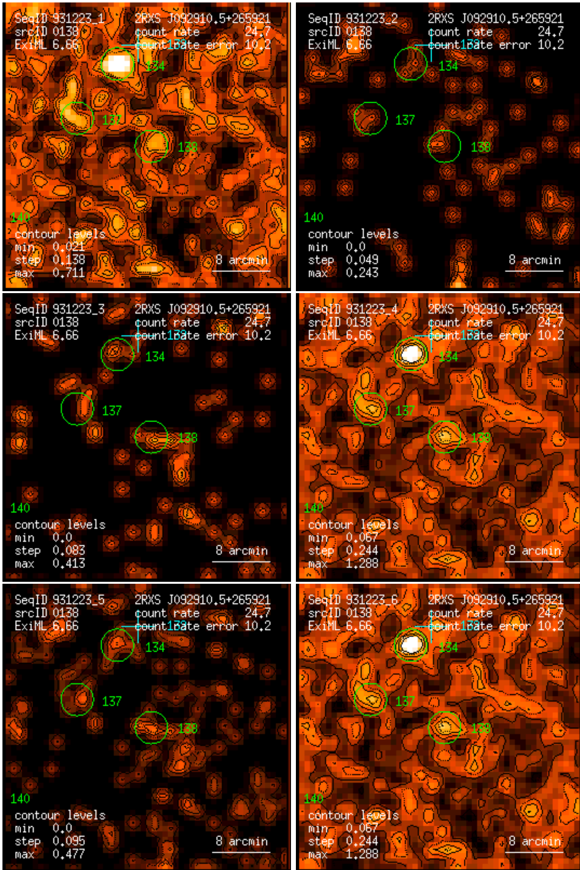
Figure 138: RASS 931223: detection 0138: band rate images, Gaussian filter: (1) PSPC channels 11 – 41, (2) 52 – 90, (3) 91 – 201, (4) 11 – 235, (5) 52 – 201, (6) 11 – 201. Broad band rates in counts/ks. Band rate contour levels in counts/ks/arcmin 2 .
