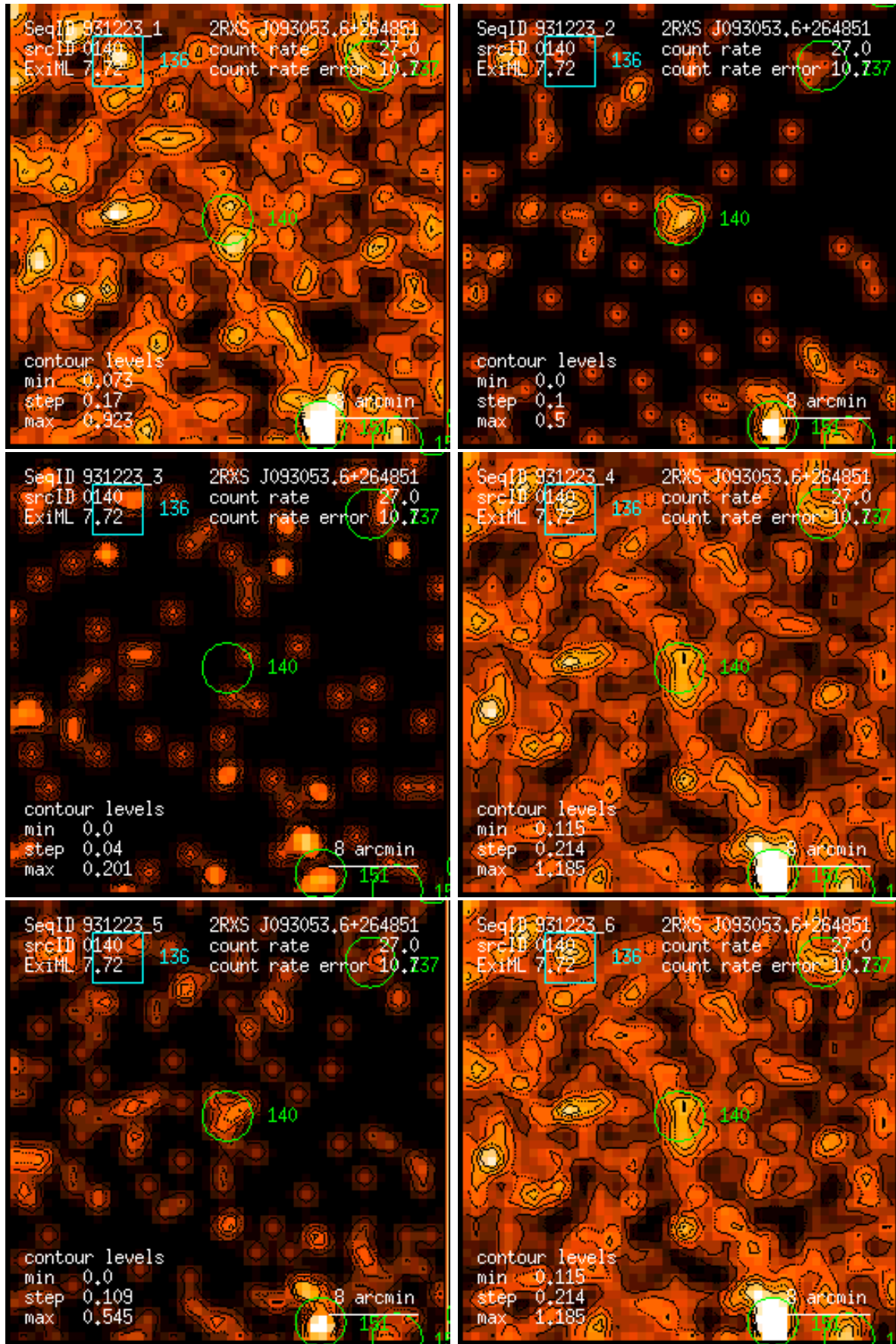
Figure 140: RASS 931223: detection 0140: band rate images, Gaussian filter: (1) PSPC channels 11 – 41, (2) 52 – 90, (3) 91 – 201, (4) 11 – 235, (5) 52 – 201, (6) 11 – 201. Broad band rates in counts/ks. Band rate contour levels in counts/ks/arcmin 2 .
