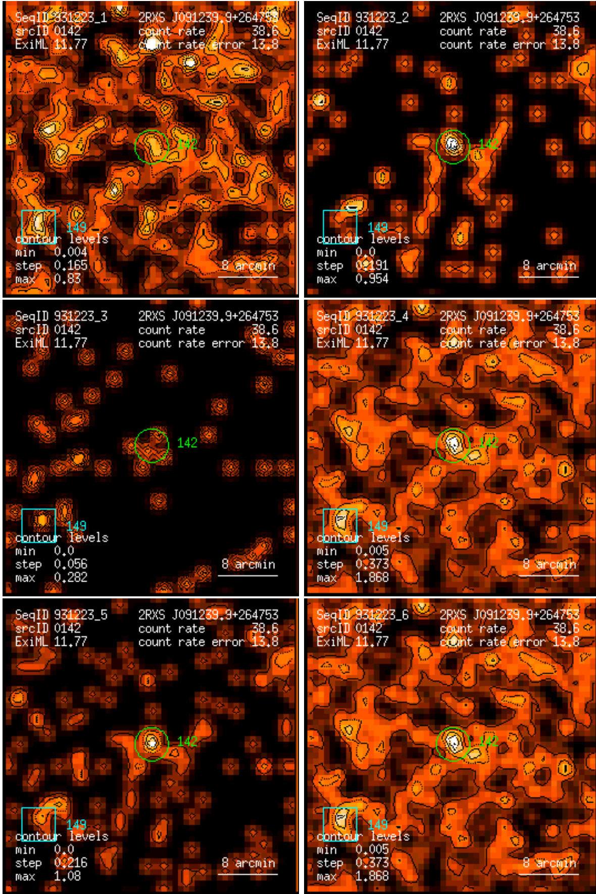
Figure 142: RASS 931223: detection 0142: band rate images, Gaussian filter: (1) PSPC channels 11 – 41, (2) 52 – 90, (3) 91 – 201, (4) 11 – 235, (5) 52 – 201, (6) 11 – 201. Broad band rates in counts/ks. Band rate contour levels in counts/ks/arcmin 2 .
