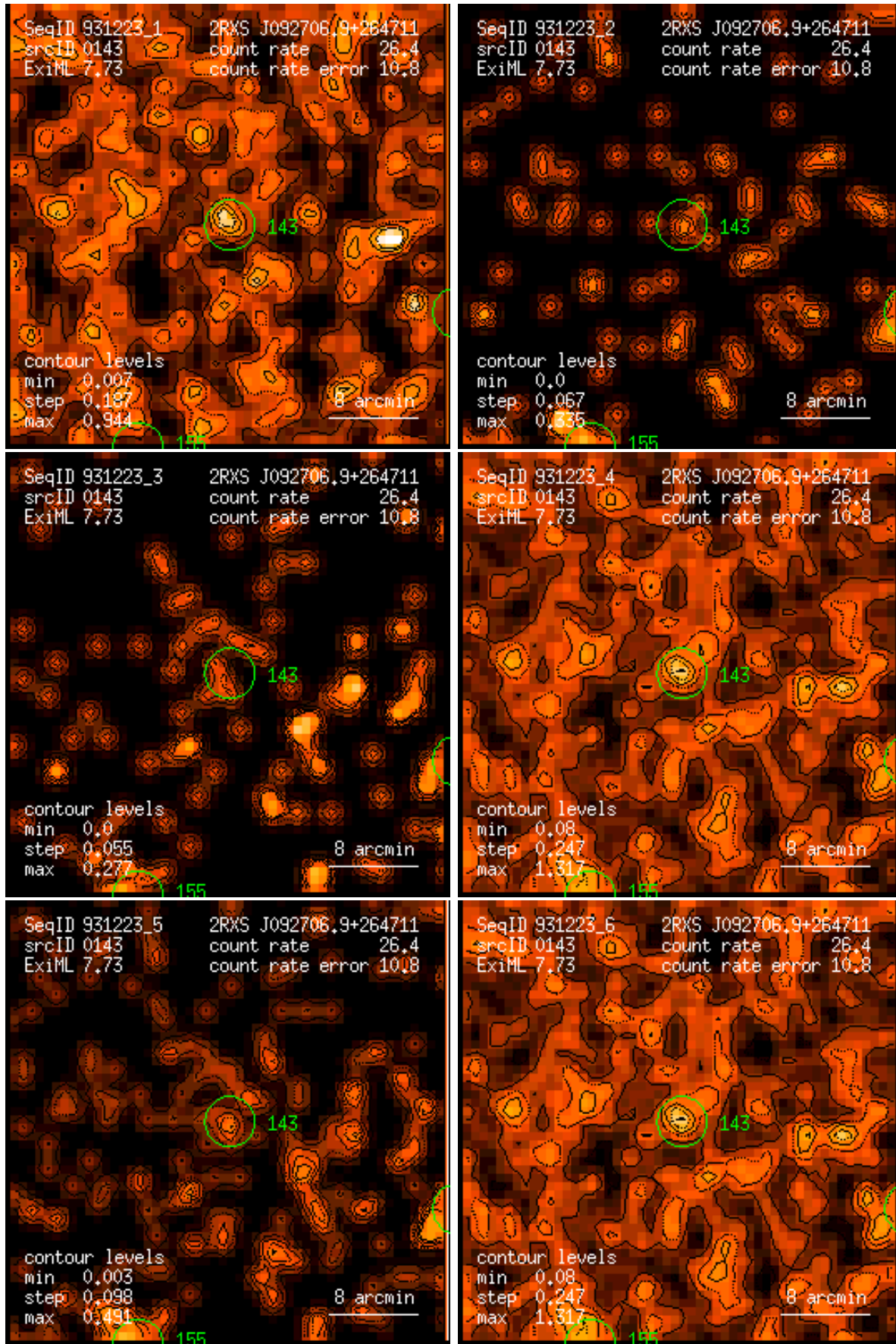
Figure 143: RASS 931223: detection 0143: band rate images, Gaussian filter: (1) PSPC channels 11 – 41, (2) 52 – 90, (3) 91 – 201, (4) 11 – 235, (5) 52 – 201, (6) 11 – 201. Broad band rates in counts/ks. Band rate contour levels in counts/ks/arcmin 2 .
