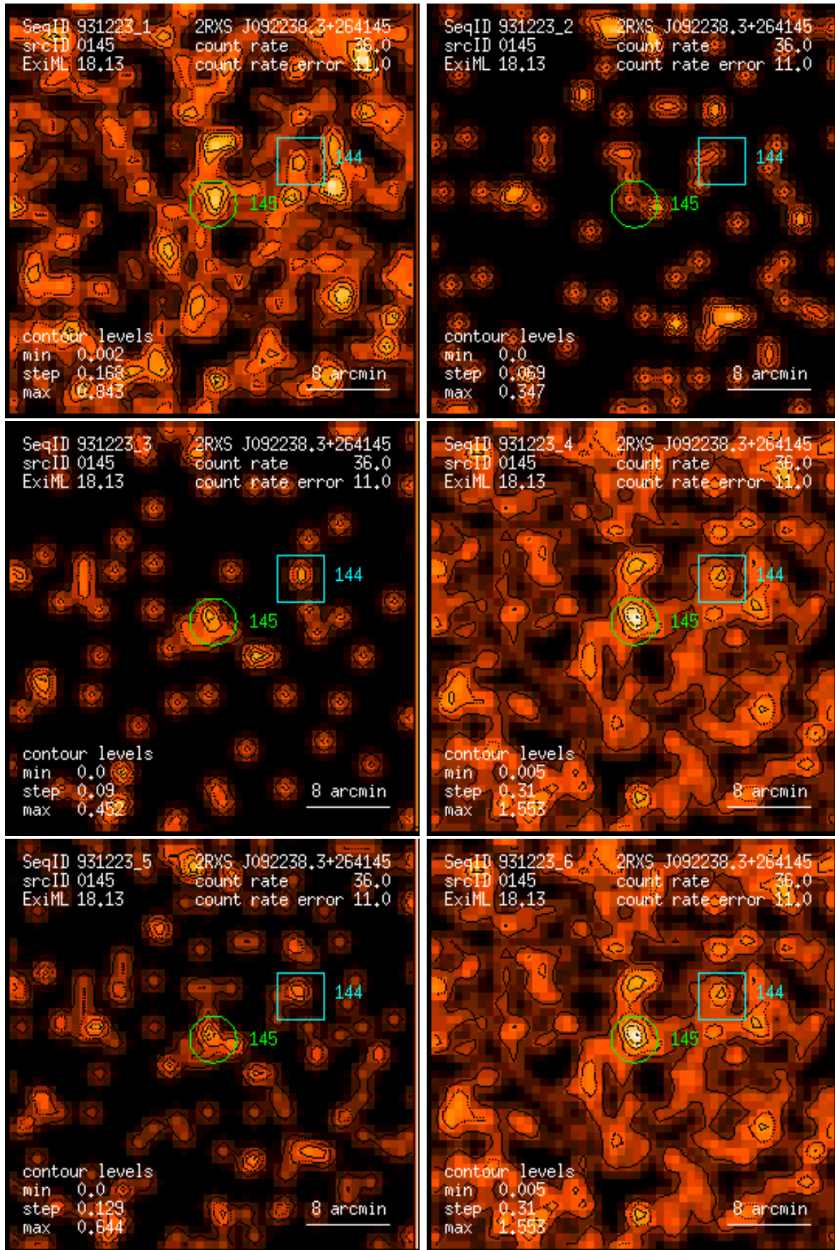
Figure 145: RASS 931223: detection 0145: band rate images, Gaussian filter: (1) PSPC channels 11 – 41, (2) 52 – 90, (3) 91 – 201, (4) 11 – 235, (5) 52 – 201, (6) 11 – 201. Broad band rates in counts/ks. Band rate contour levels in counts/ks/arcmin 2 .
