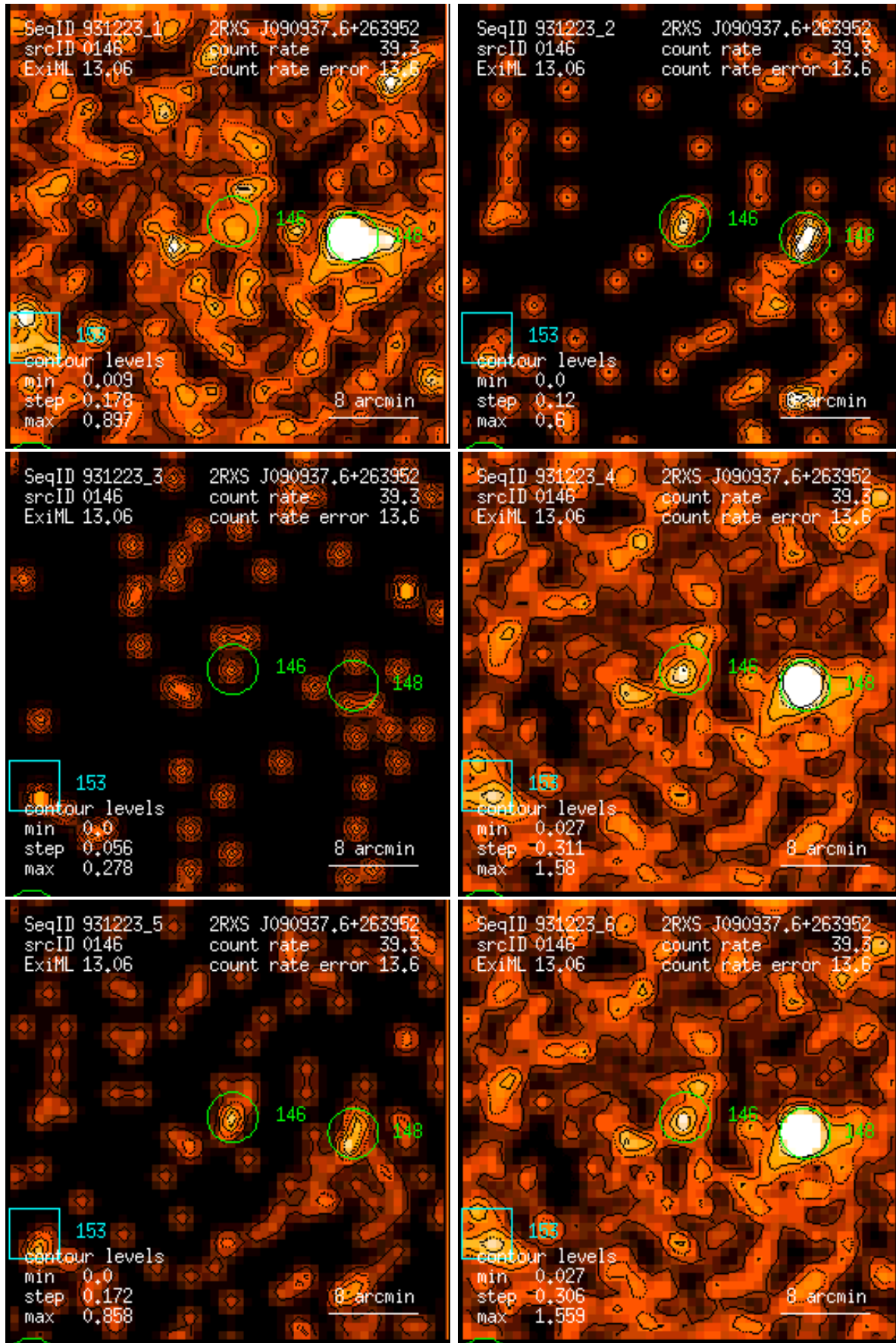
Figure 146: RASS 931223: detection 0146: band rate images, Gaussian filter: (1) PSPC channels 11 – 41, (2) 52 – 90, (3) 91 – 201, (4) 11 – 235, (5) 52 – 201, (6) 11 – 201. Broad band rates in counts/ks. Band rate contour levels in counts/ks/arcmin 2 .
