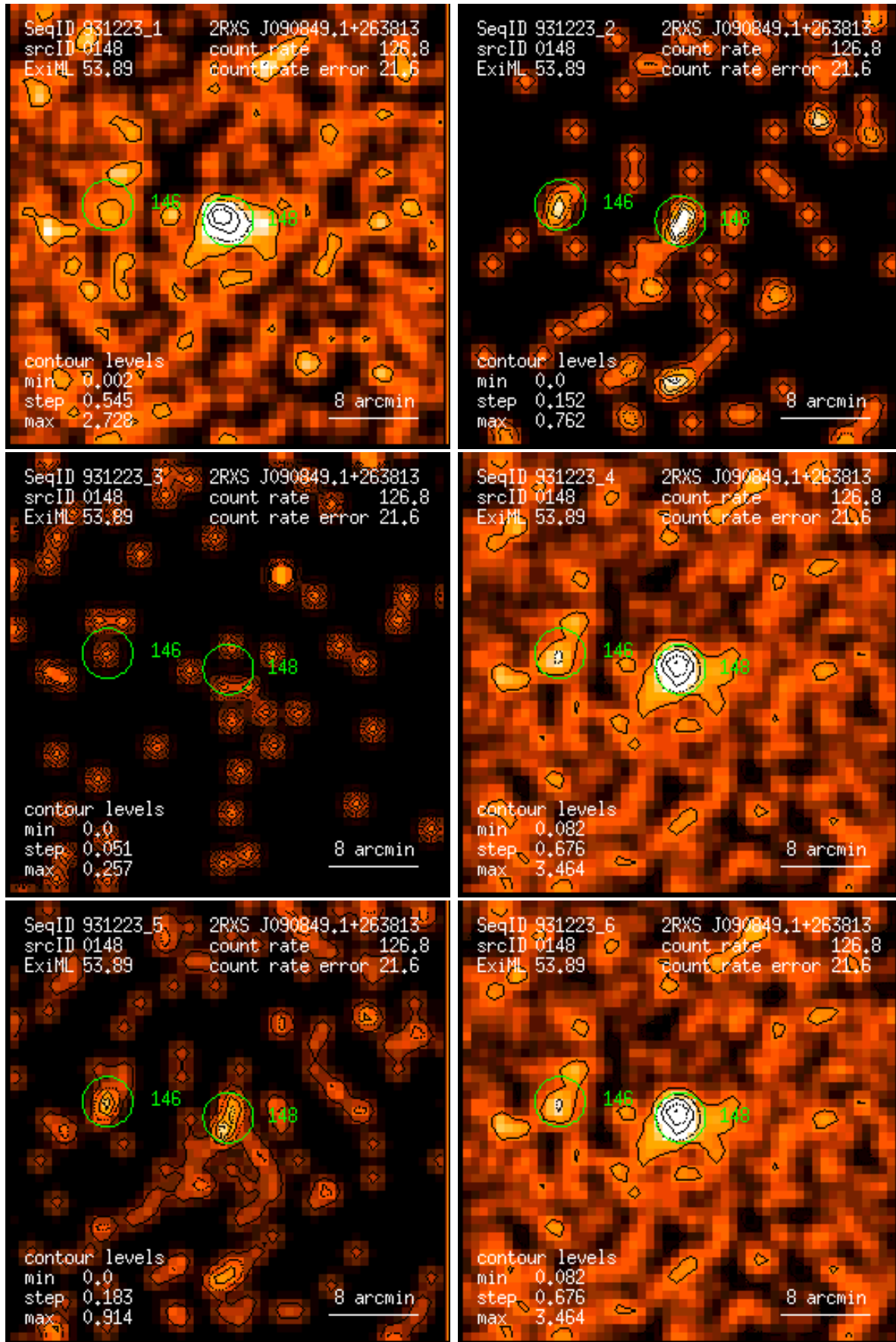
Figure 148: RASS 931223: detection 0148: band rate images, Gaussian filter: (1) PSPC channels 11 – 41, (2) 52 – 90, (3) 91 – 201, (4) 11 – 235, (5) 52 – 201, (6) 11 – 201. Broad band rates in counts/ks. Band rate contour levels in counts/ks/arcmin 2 .
