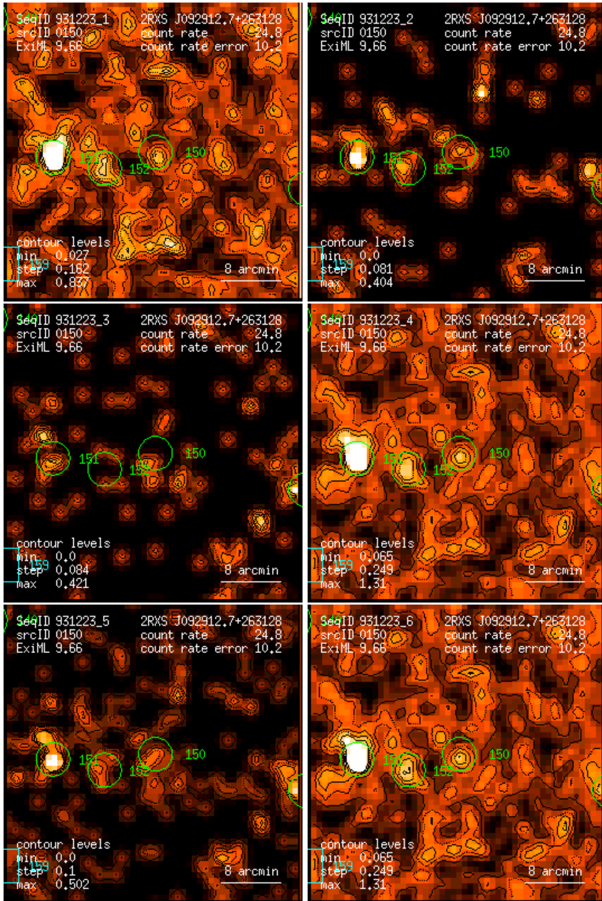
Figure 150: RASS 931223: detection 0150: band rate images, Gaussian filter: (1) PSPC channels 11 – 41, (2) 52 – 90, (3) 91 – 201, (4) 11 – 235, (5) 52 – 201, (6) 11 – 201. Broad band rates in counts/ks. Band rate contour levels in counts/ks/arcmin 2 .
