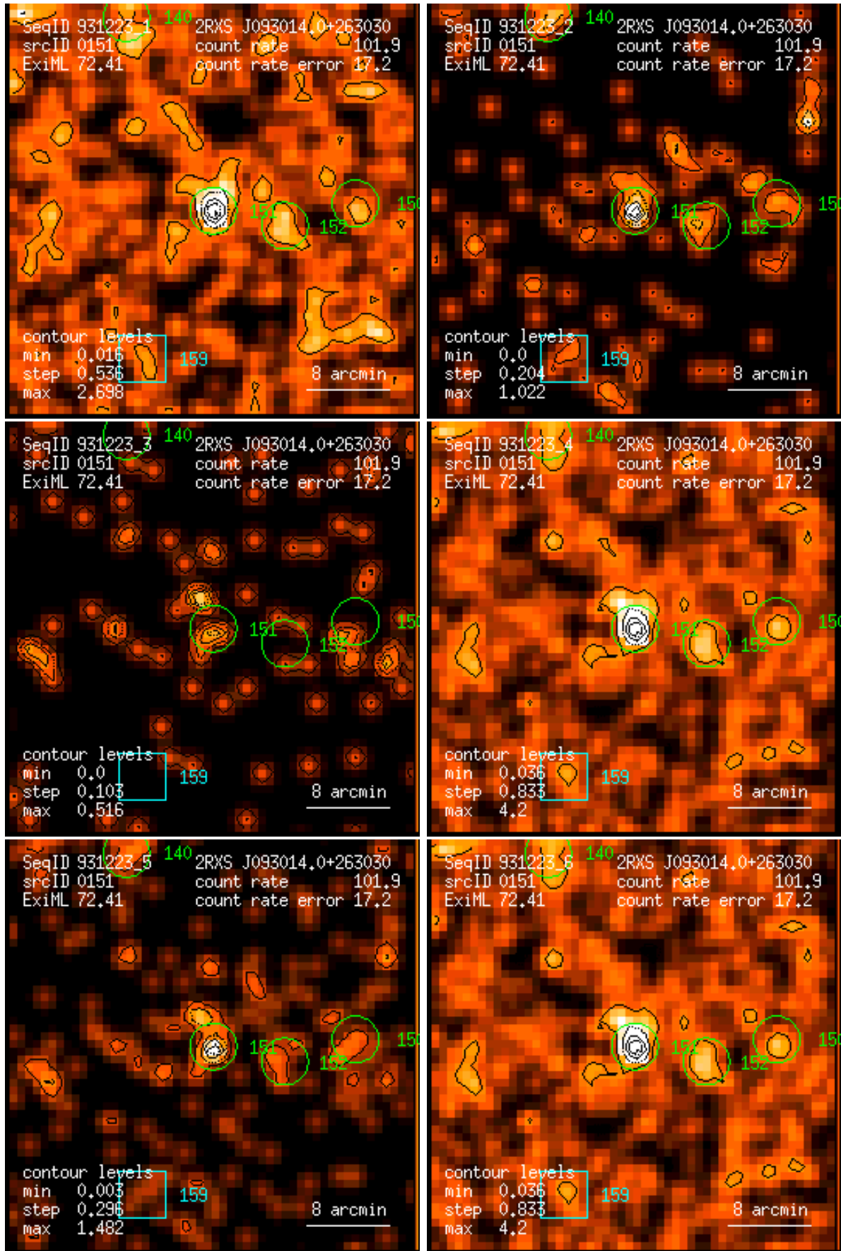
Figure 151: RASS 931223: detection 0151: band rate images, Gaussian filter: (1) PSPC channels 11 – 41, (2) 52 – 90, (3) 91 – 201, (4) 11 – 235, (5) 52 – 201, (6) 11 – 201. Broad band rates in counts/ks. Band rate contour levels in counts/ks/arcmin 2 .
