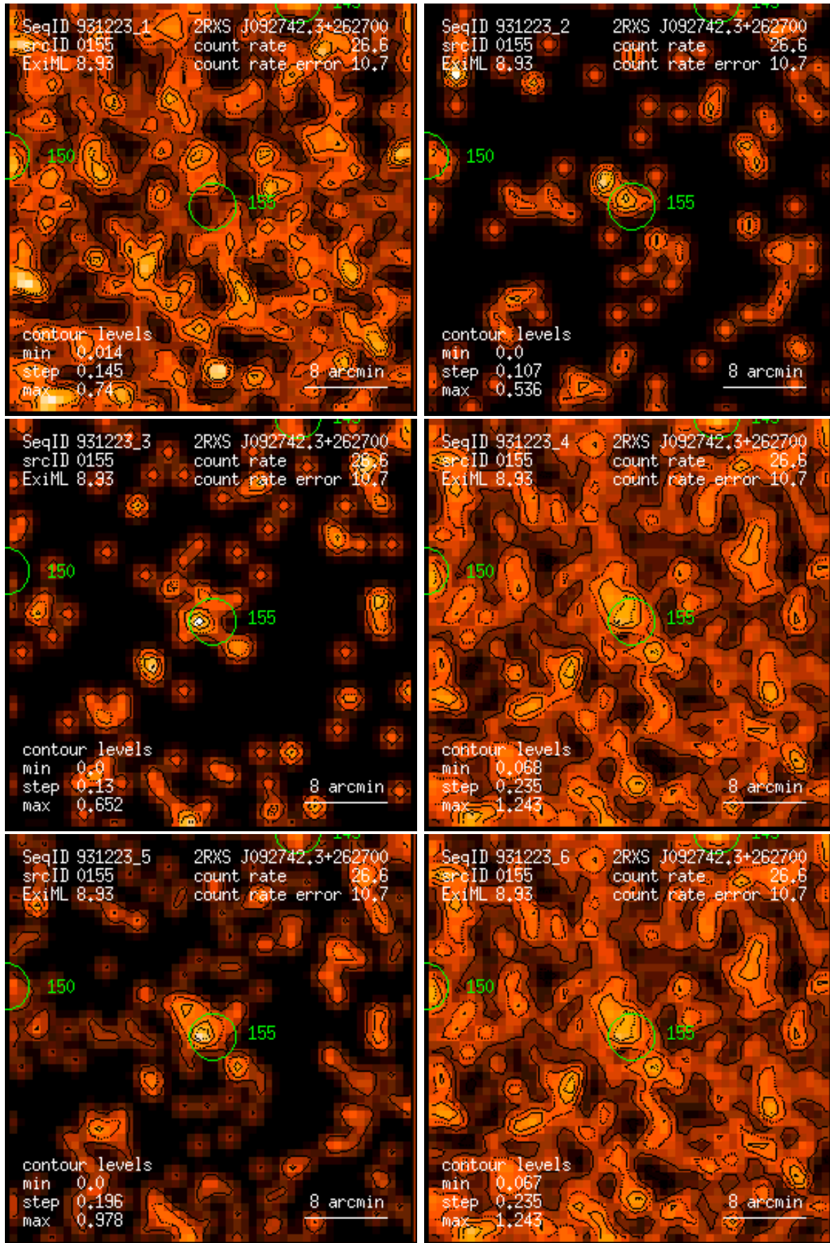
Figure 155: RASS 931223: detection 0155: band rate images, Gaussian filter: (1) PSPC channels 11 – 41, (2) 52 – 90, (3) 91 – 201, (4) 11 – 235, (5) 52 – 201, (6) 11 – 201. Broad band rates in counts/ks. Band rate contour levels in counts/ks/arcmin 2 .
