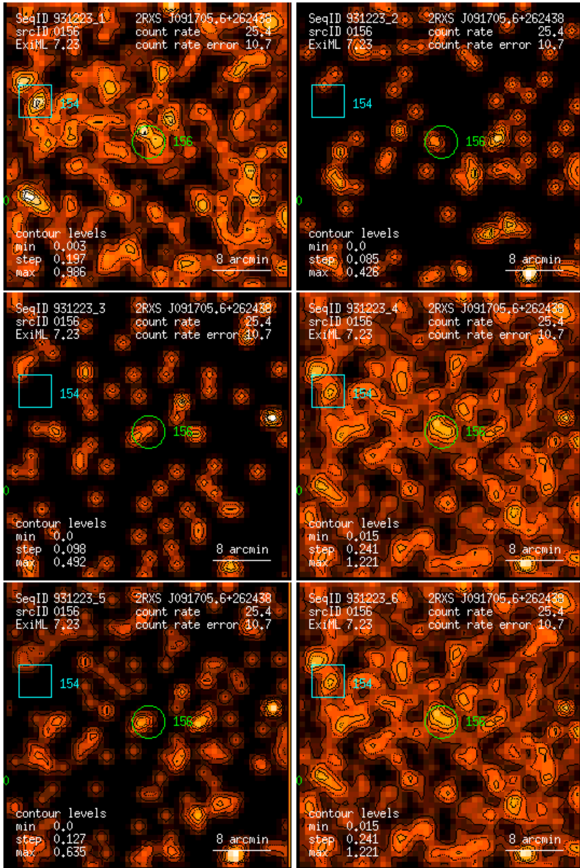
Figure 156: RASS 931223: detection 0156: band rate images, Gaussian filter: (1) PSPC channels 11 – 41, (2) 52 – 90, (3) 91 – 201, (4) 11 – 235, (5) 52 – 201, (6) 11 – 201. Broad band rates in counts/ks. Band rate contour levels in counts/ks/arcmin 2 .
