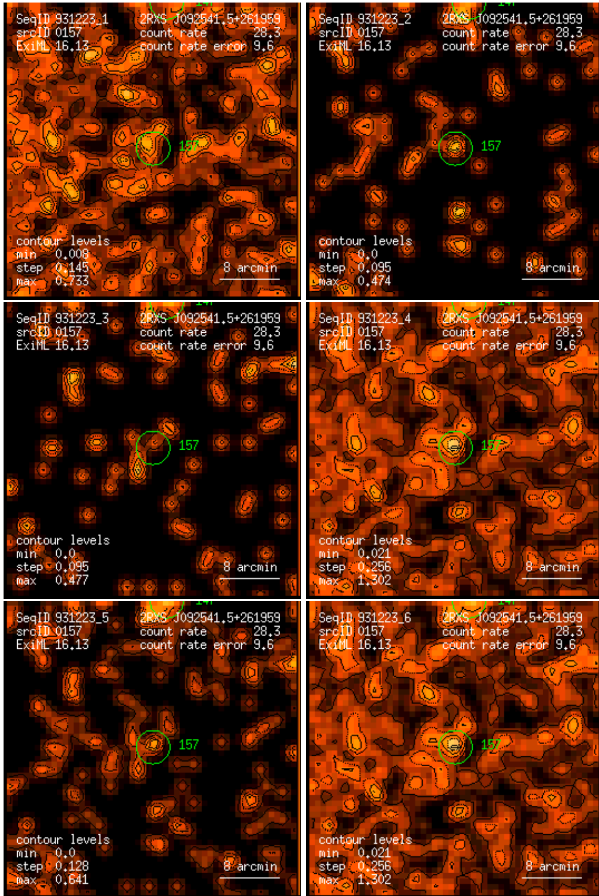
Figure 157: RASS 931223: detection 0157: band rate images, Gaussian filter: (1) PSPC channels 11 – 41, (2) 52 – 90, (3) 91 – 201, (4) 11 – 235, (5) 52 – 201, (6) 11 – 201. Broad band rates in counts/ks. Band rate contour levels in counts/ks/arcmin 2 .
