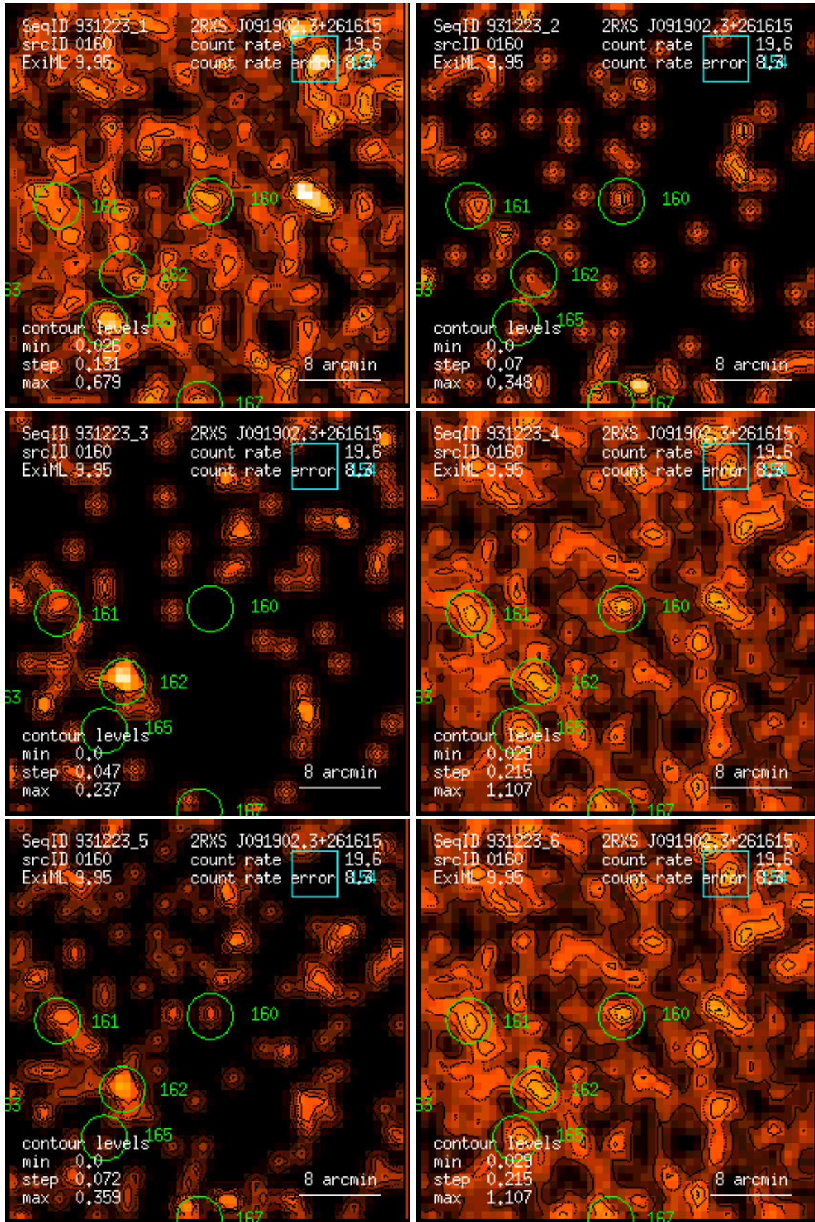
Figure 160: RASS 931223: detection 0160: band rate images, Gaussian filter: (1) PSPC channels 11 – 41, (2) 52 – 90, (3) 91 – 201, (4) 11 – 235, (5) 52 – 201, (6) 11 – 201. Broad band rates in counts/ks. Band rate contour levels in counts/ks/arcmin 2 .
