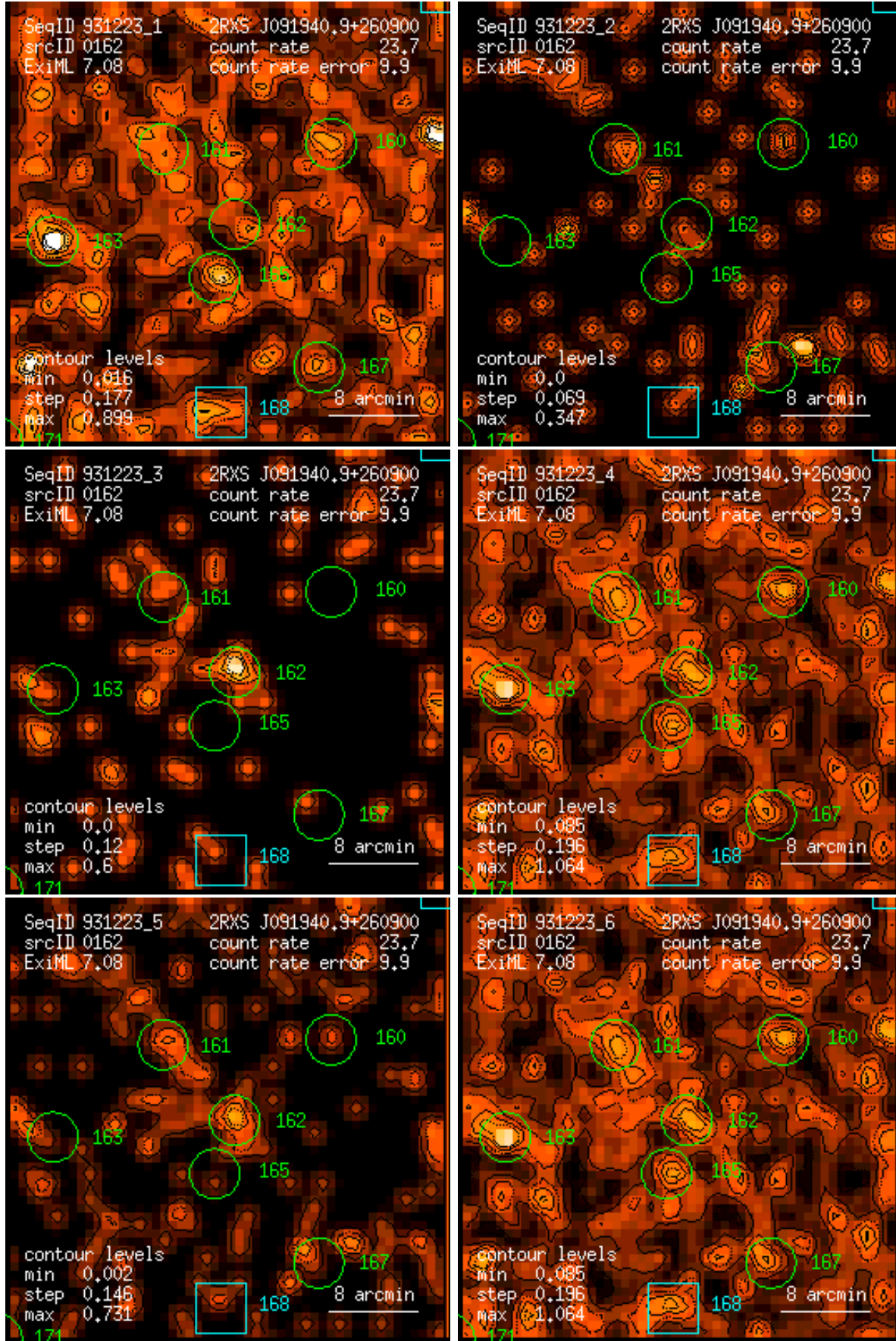
Figure 162: RASS 931223: detection 0162: band rate images, Gaussian filter: (1) PSPC channels 11 – 41, (2) 52 – 90, (3) 91 – 201, (4) 11 – 235, (5) 52 – 201, (6) 11 – 201. Broad band rates in counts/ks. Band rate contour levels in counts/ks/arcmin 2 .
