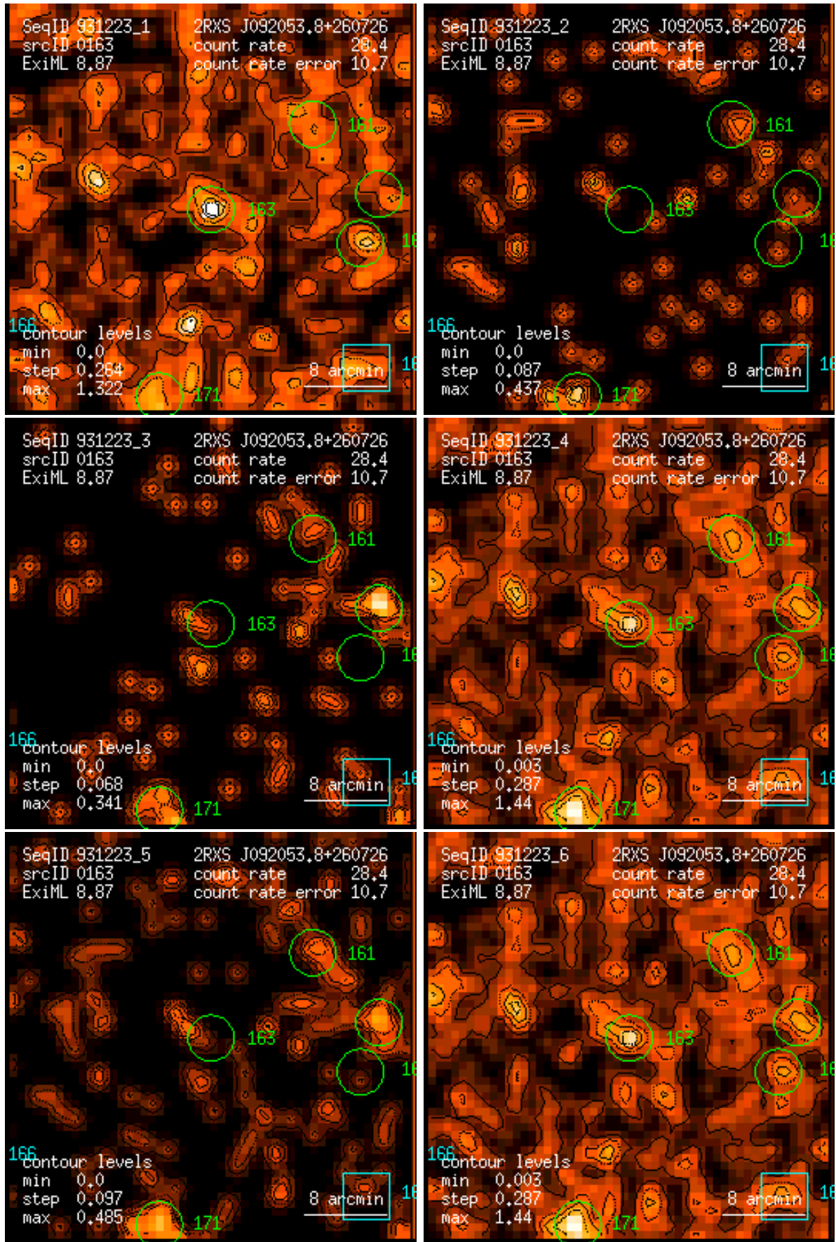
Figure 163: RASS 931223: detection 0163: band rate images, Gaussian filter: (1) PSPC channels 11 – 41, (2) 52 – 90, (3) 91 – 201, (4) 11 – 235, (5) 52 – 201, (6) 11 – 201. Broad band rates in counts/ks. Band rate contour levels in counts/ks/arcmin 2 .
