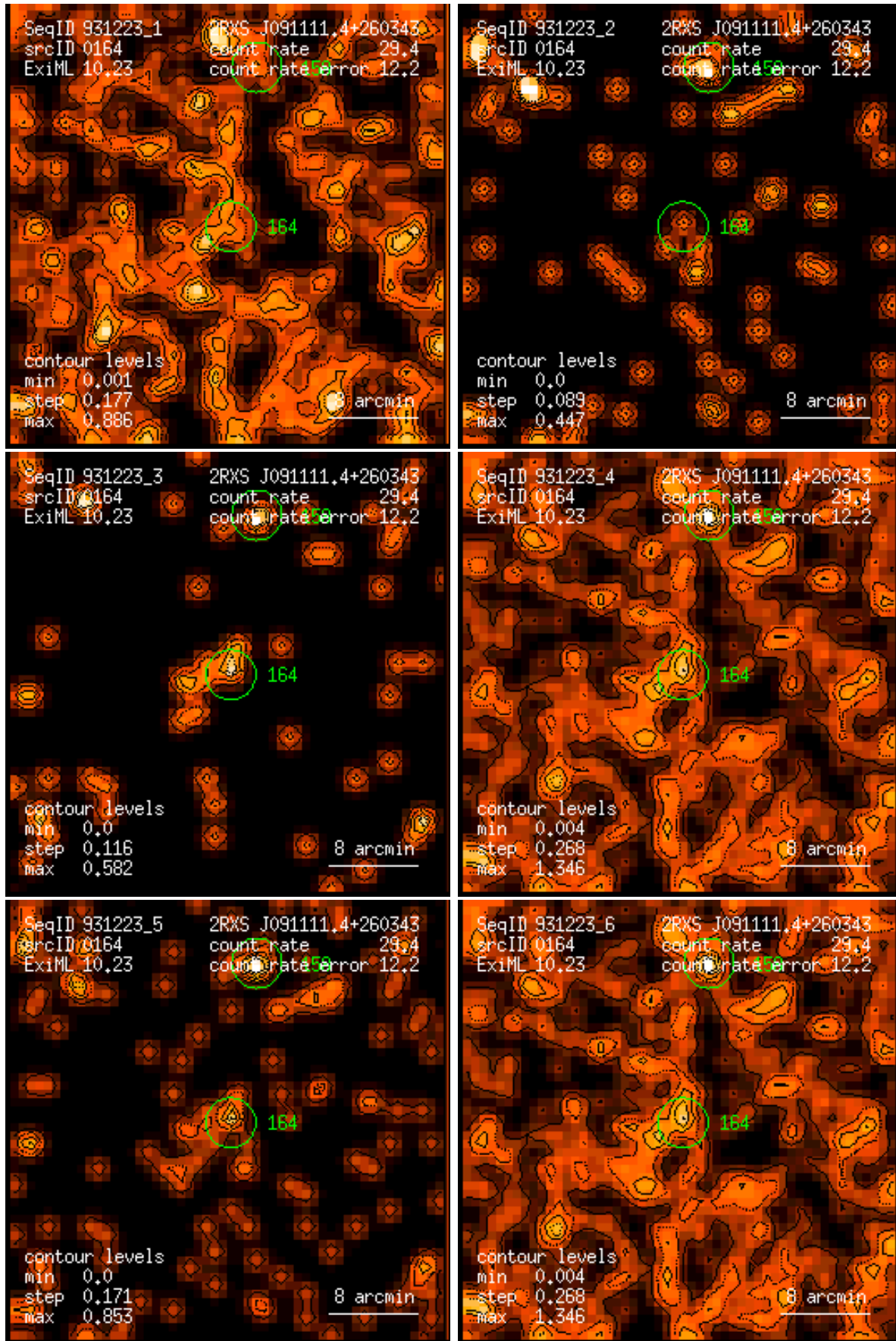
Figure 164: RASS 931223: detection 0164: band rate images, Gaussian filter: (1) PSPC channels 11 – 41, (2) 52 – 90, (3) 91 – 201, (4) 11 – 235, (5) 52 – 201, (6) 11 – 201. Broad band rates in counts/ks. Band rate contour levels in counts/ks/arcmin 2 .
