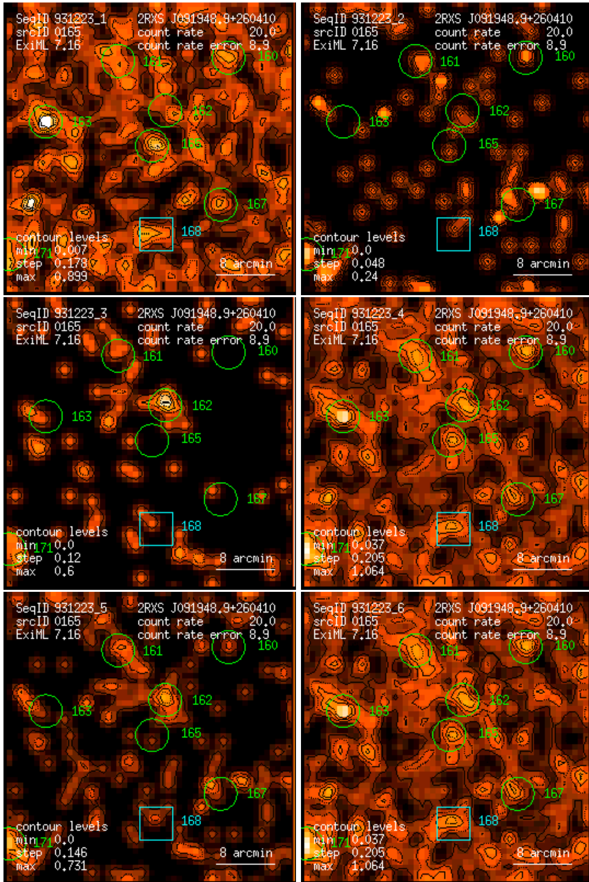
Figure 165: RASS 931223: detection 0165: band rate images, Gaussian filter: (1) PSPC channels 11 – 41, (2) 52 – 90, (3) 91 – 201, (4) 11 – 235, (5) 52 – 201, (6) 11 – 201. Broad band rates in counts/ks. Band rate contour levels in counts/ks/arcmin 2 .
