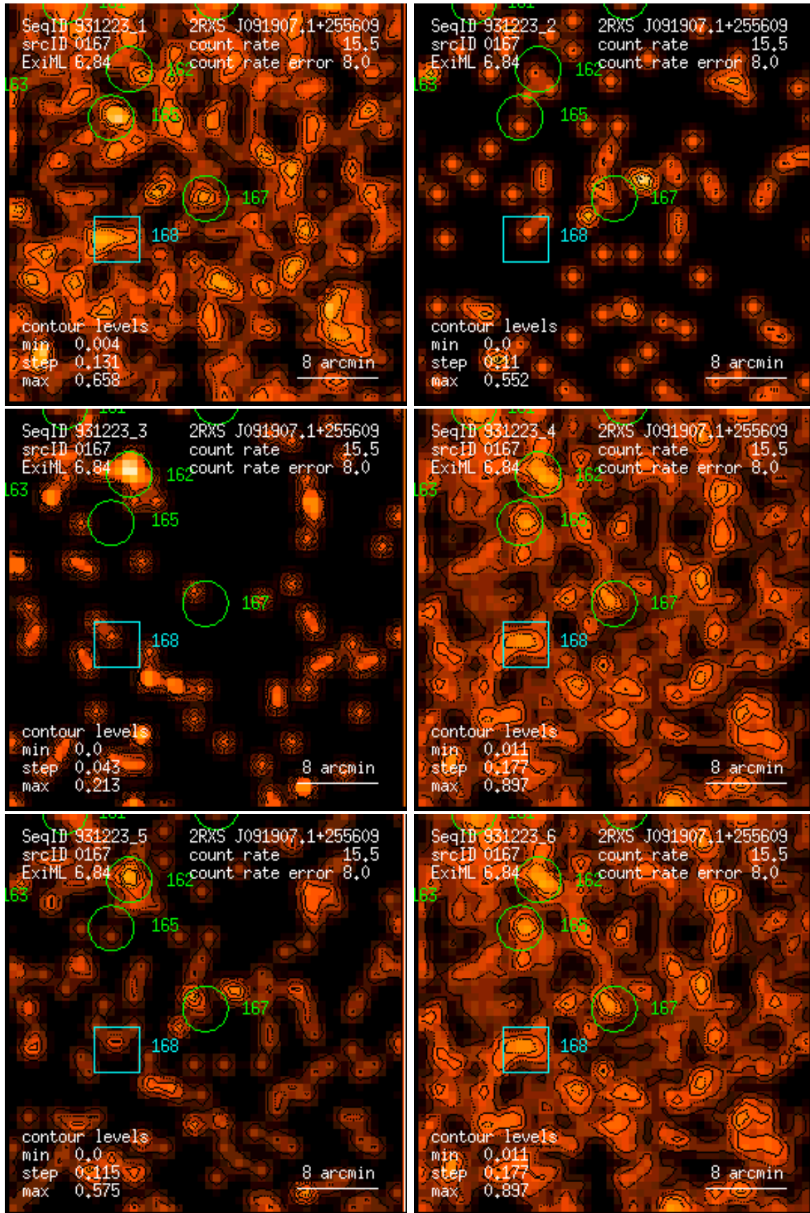
Figure 167: RASS 931223: detection 0167: band rate images, Gaussian filter: (1) PSPC channels 11 – 41, (2) 52 – 90, (3) 91 – 201, (4) 11 – 235, (5) 52 – 201, (6) 11 – 201. Broad band rates in counts/ks. Band rate contour levels in counts/ks/arcmin 2 .
