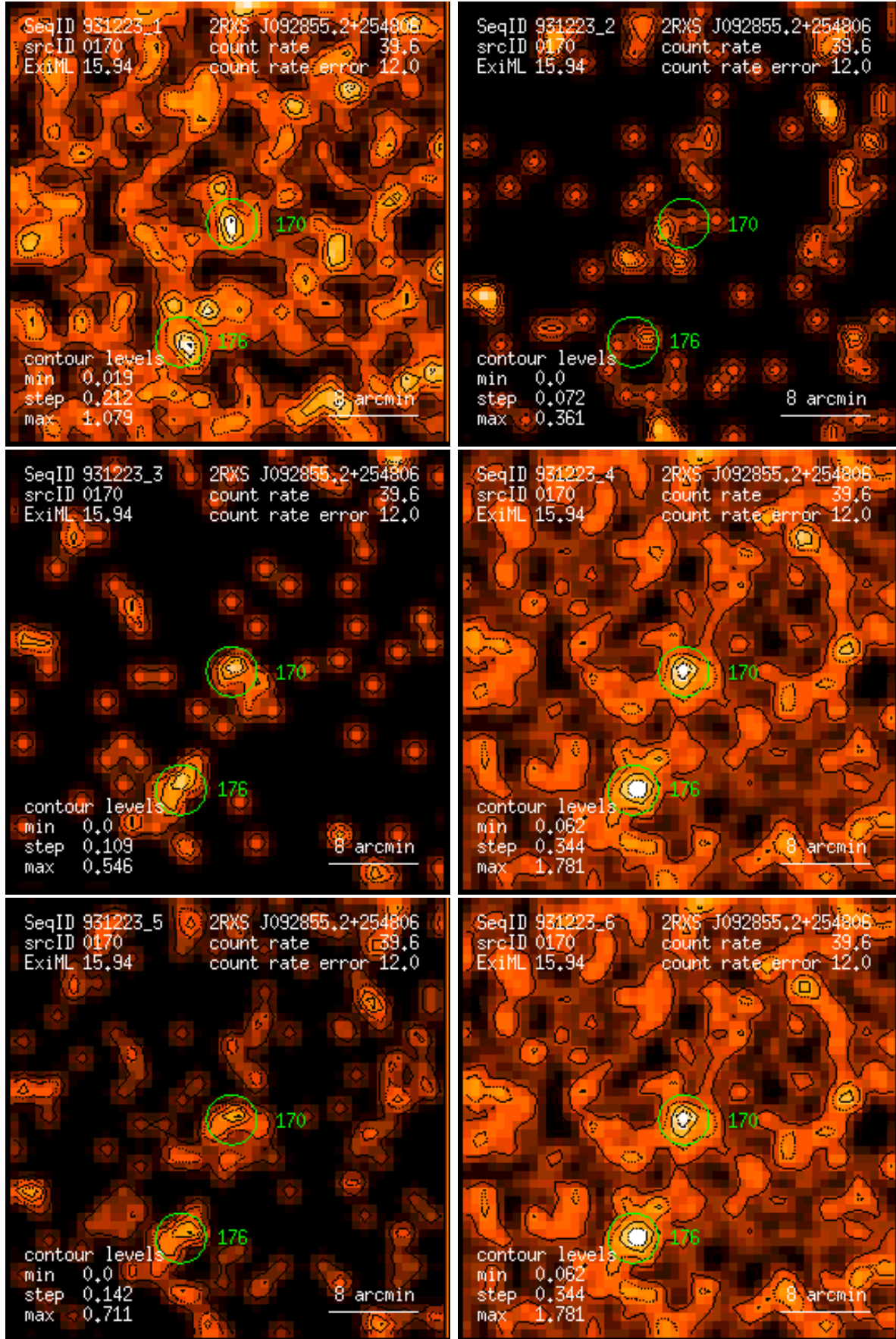
Figure 170: RASS 931223: detection 0170: band rate images, Gaussian filter: (1) PSPC channels 11 – 41, (2) 52 – 90, (3) 91 – 201, (4) 11 – 235, (5) 52 – 201, (6) 11 – 201. Broad band rates in counts/ks. Band rate contour levels in counts/ks/arcmin 2 .
