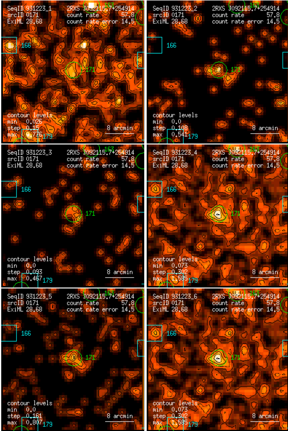
Figure 171: RASS 931223: detection 0171: band rate images, Gaussian filter: (1) PSPC channels 11 – 41, (2) 52 – 90, (3) 91 – 201, (4) 11 – 235, (5) 52 – 201, (6) 11 – 201. Broad band rates in counts/ks. Band rate contour levels in counts/ks/arcmin 2 .
