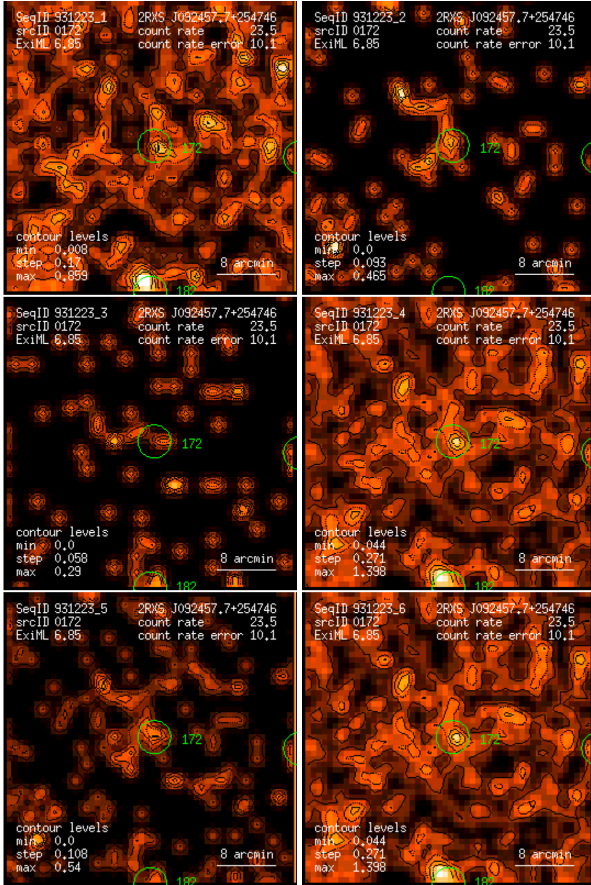
Figure 172: RASS 931223: detection 0172: band rate images, Gaussian filter: (1) PSPC channels 11 – 41, (2) 52 – 90, (3) 91 – 201, (4) 11 – 235, (5) 52 – 201, (6) 11 – 201. Broad band rates in counts/ks. Band rate contour levels in counts/ks/arcmin 2 .
