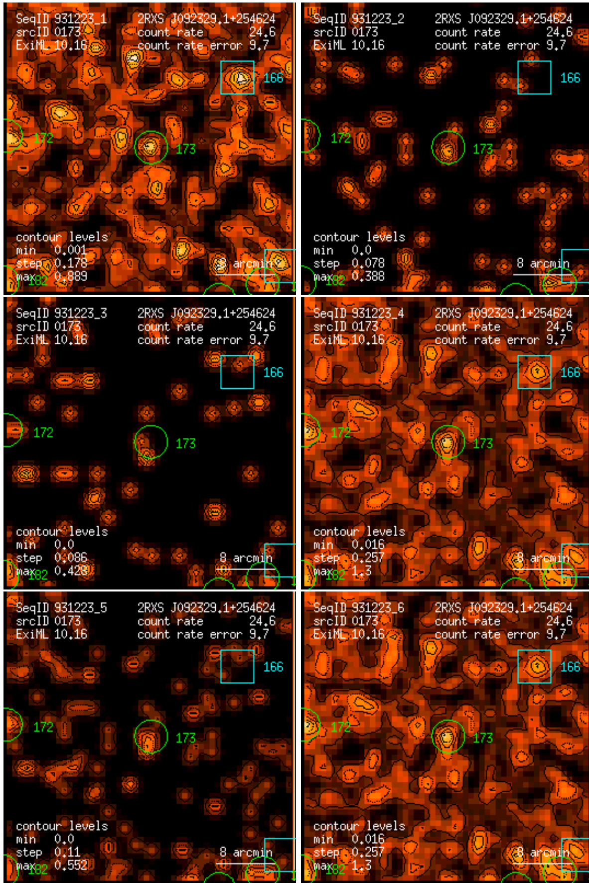
Figure 173: RASS 931223: detection 0173: band rate images, Gaussian filter: (1) PSPC channels 11 – 41, (2) 52 – 90, (3) 91 – 201, (4) 11 – 235, (5) 52 – 201, (6) 11 – 201. Broad band rates in counts/ks. Band rate contour levels in counts/ks/arcmin 2 .
