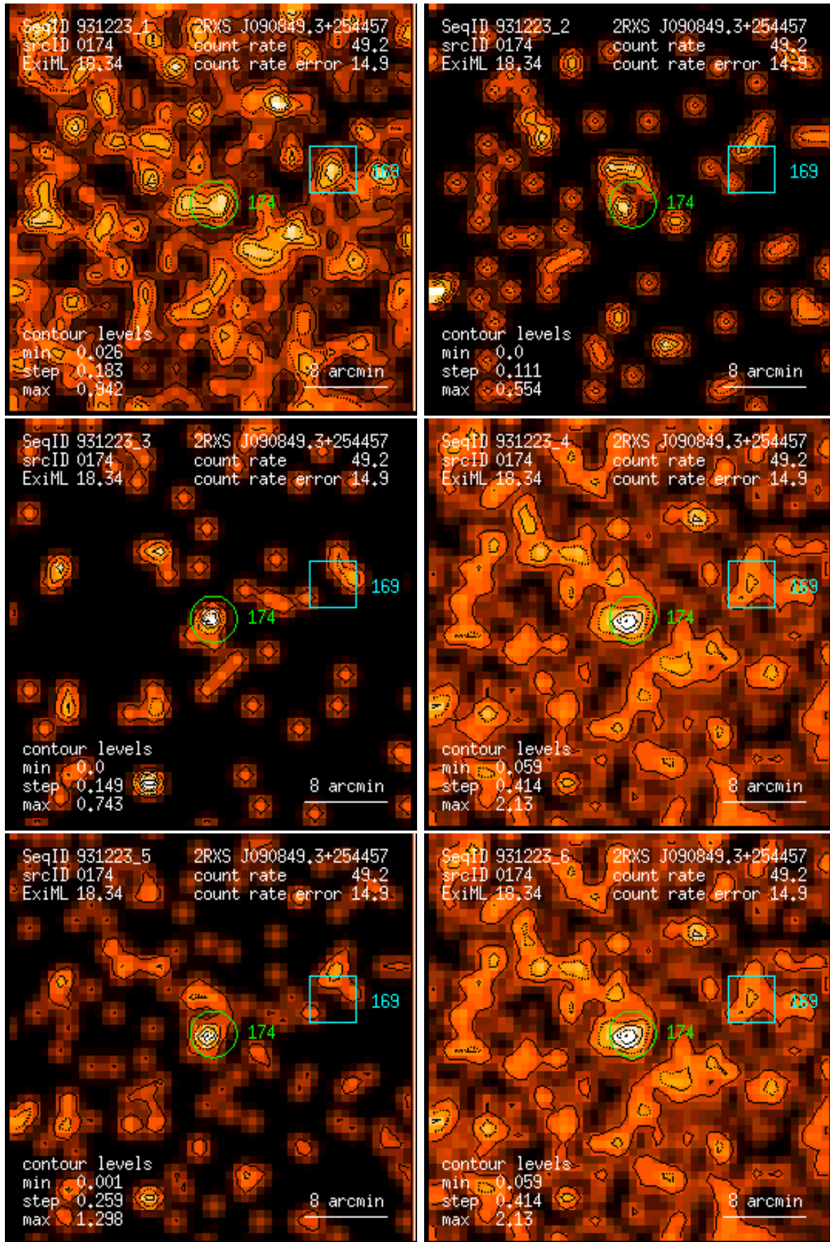
Figure 174: RASS 931223: detection 0174: band rate images, Gaussian filter: (1) PSPC channels 11 – 41, (2) 52 – 90, (3) 91 – 201, (4) 11 – 235, (5) 52 – 201, (6) 11 – 201. Broad band rates in counts/ks. Band rate contour levels in counts/ks/arcmin 2 .
