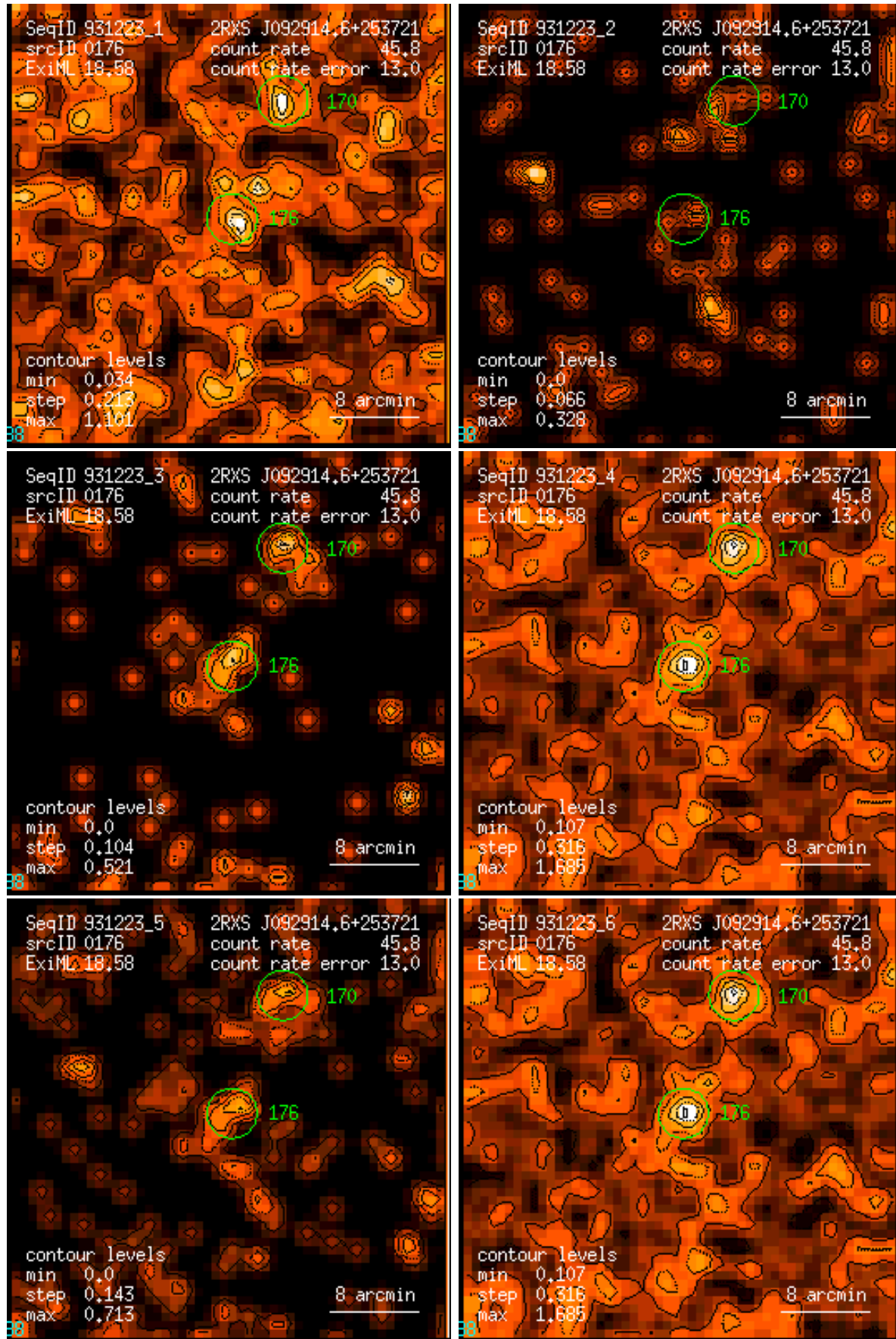
Figure 176: RASS 931223: detection 0176: band rate images, Gaussian filter: (1) PSPC channels 11 – 41, (2) 52 – 90, (3) 91 – 201, (4) 11 – 235, (5) 52 – 201, (6) 11 – 201. Broad band rates in counts/ks. Band rate contour levels in counts/ks/arcmin 2 .
