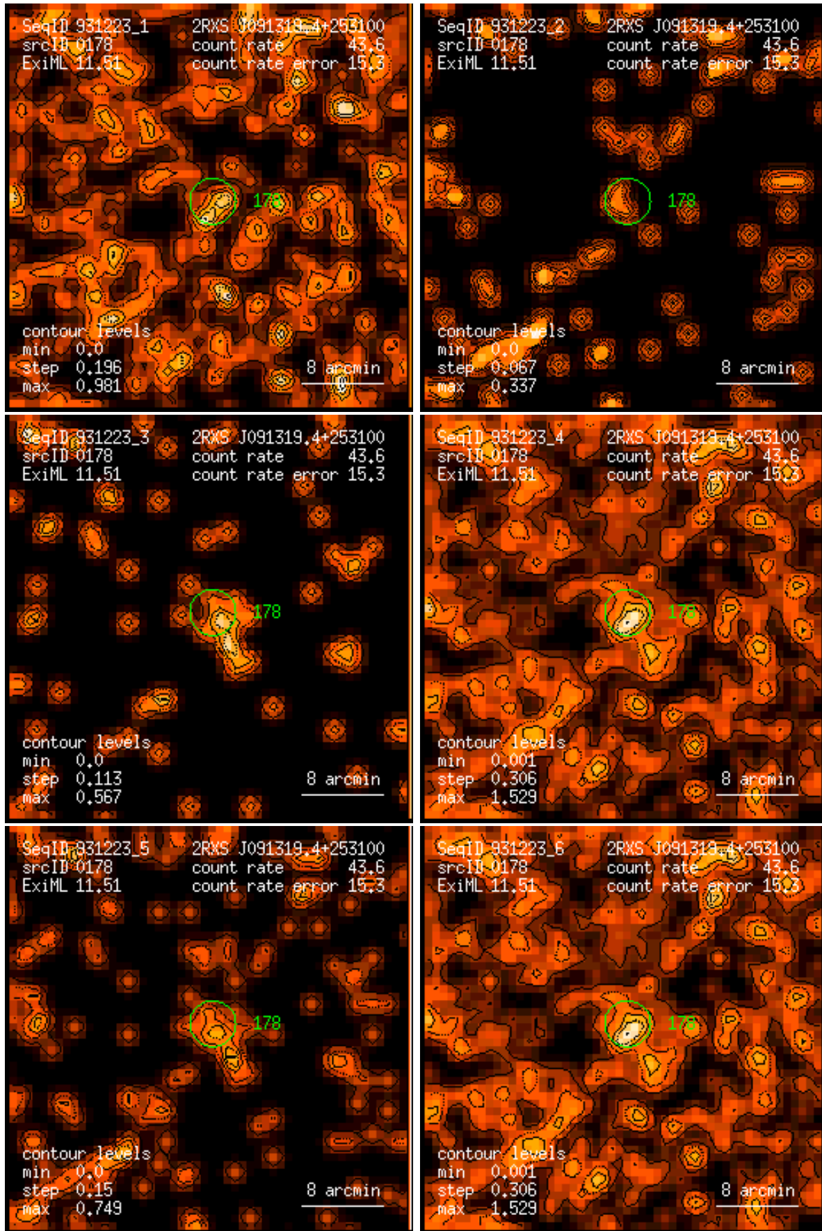
Figure 178: RASS 931223: detection 0178: band rate images, Gaussian filter: (1) PSPC channels 11 – 41, (2) 52 – 90, (3) 91 – 201, (4) 11 – 235, (5) 52 – 201, (6) 11 – 201. Broad band rates in counts/ks. Band rate contour levels in counts/ks/arcmin 2 .
