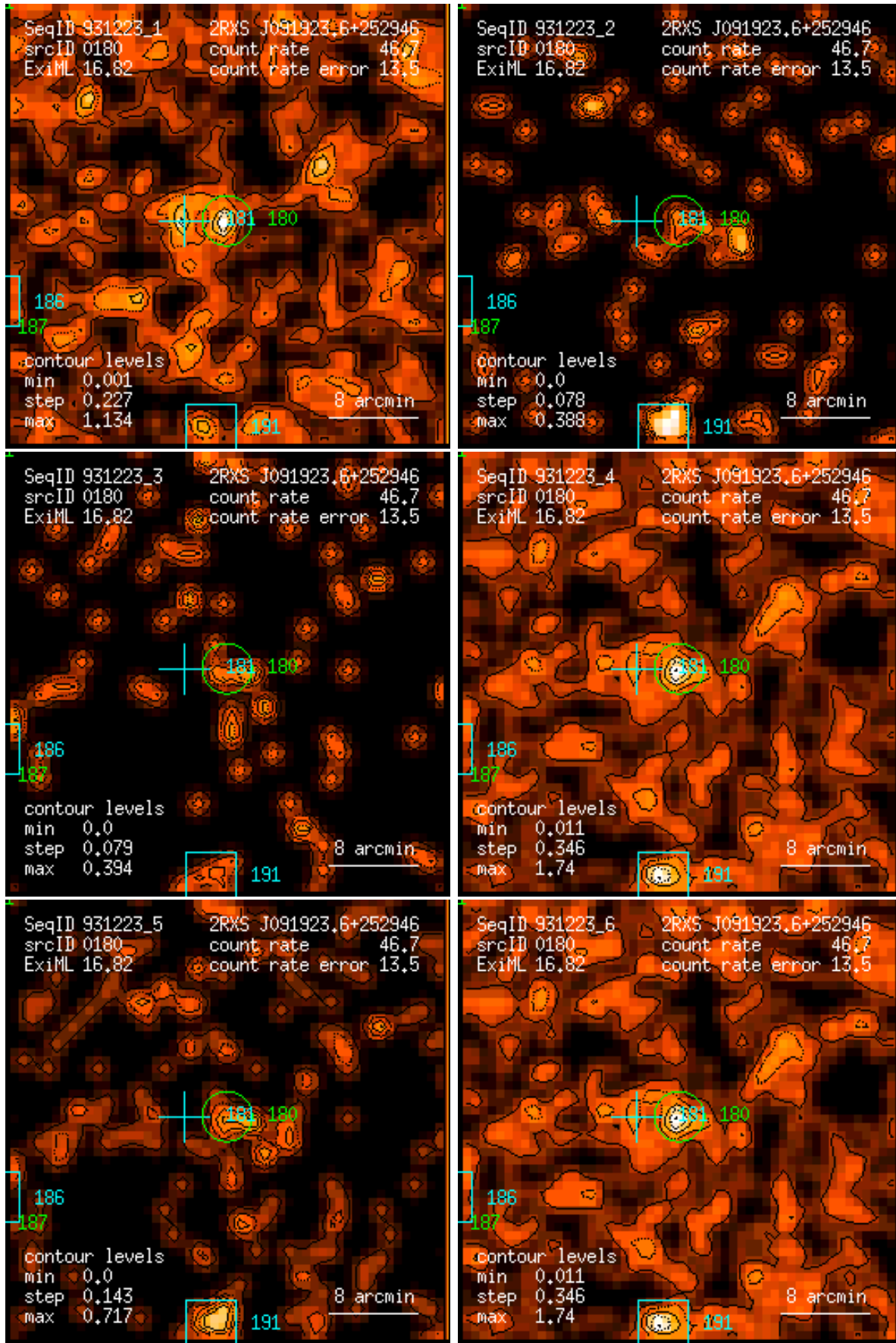
Figure 180: RASS 931223: detection 0180: band rate images, Gaussian filter: (1) PSPC channels 11 – 41, (2) 52 – 90, (3) 91 – 201, (4) 11 – 235, (5) 52 – 201, (6) 11 – 201. Broad band rates in counts/ks. Band rate contour levels in counts/ks/arcmin 2 .
