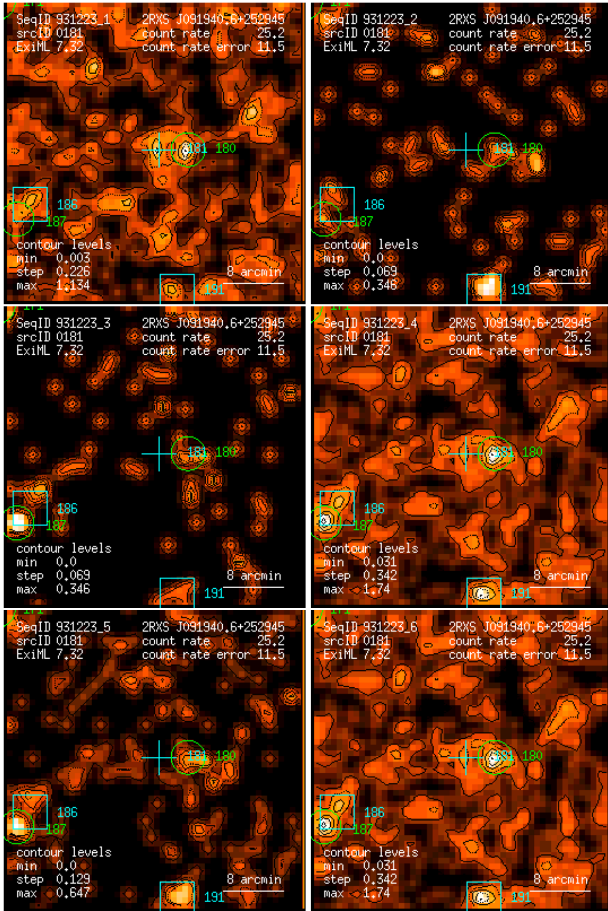
Figure 181: RASS 931223: detection 0181: band rate images, Gaussian filter: (1) PSPC channels 11 – 41, (2) 52 – 90, (3) 91 – 201, (4) 11 – 235, (5) 52 – 201, (6) 11 – 201. Broad band rates in counts/ks. Band rate contour levels in counts/ks/arcmin 2 .
