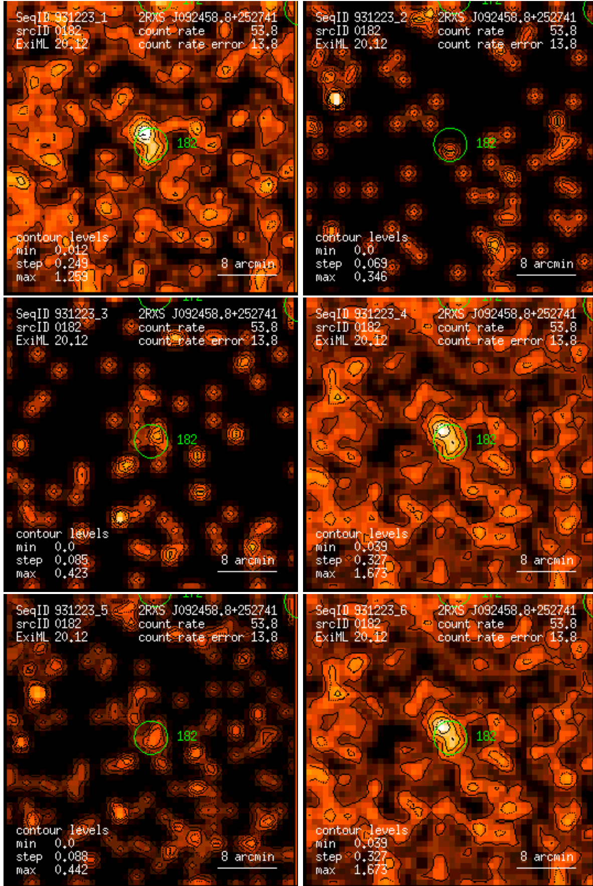
Figure 182: RASS 931223: detection 0182: band rate images, Gaussian filter: (1) PSPC channels 11 – 41, (2) 52 – 90, (3) 91 – 201, (4) 11 – 235, (5) 52 – 201, (6) 11 – 201. Broad band rates in counts/ks. Band rate contour levels in counts/ks/arcmin 2 .
