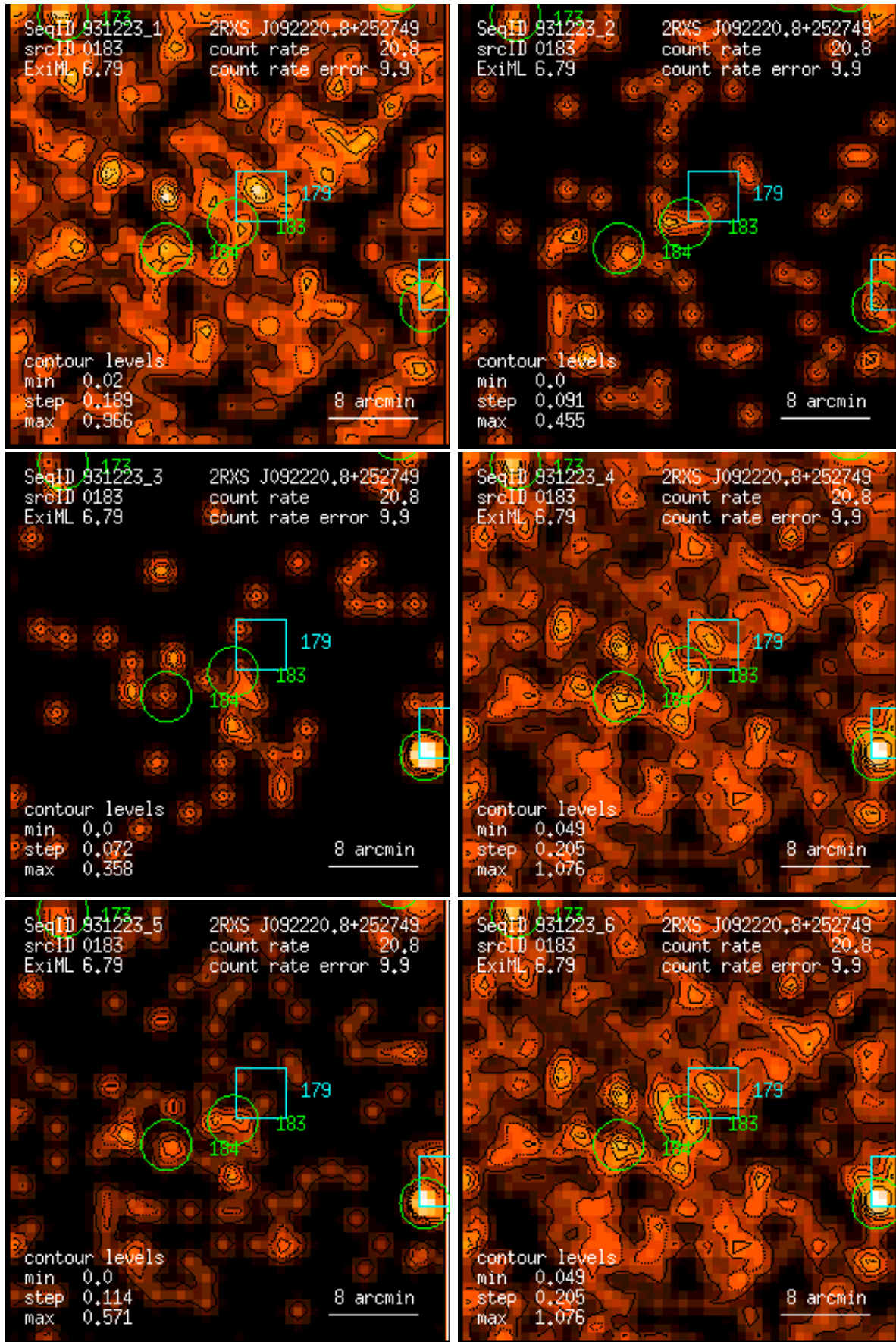
Figure 183: RASS 931223: detection 0183: band rate images, Gaussian filter: (1) PSPC channels 11 – 41, (2) 52 – 90, (3) 91 – 201, (4) 11 – 235, (5) 52 – 201, (6) 11 – 201. Broad band rates in counts/ks. Band rate contour levels in counts/ks/arcmin 2 .
