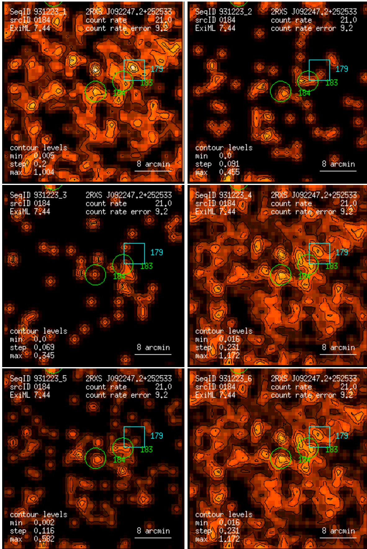
Figure 184: RASS 931223: detection 0184: band rate images, Gaussian filter: (1) PSPC channels 11 – 41, (2) 52 – 90, (3) 91 – 201, (4) 11 – 235, (5) 52 – 201, (6) 11 – 201. Broad band rates in counts/ks. Band rate contour levels in counts/ks/arcmin 2 .
